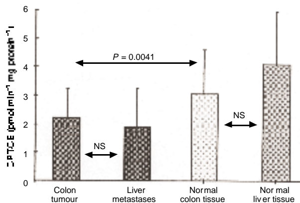
Figure 2 Comparison of CPT-11 converting carboxylase (CPT-CE) activity in tumour and normal tissues. No difference between tumour colon tissue and liver metastases or between colon and liver normal tissues. (NS) Significant difference between tumour and normal colon tissue (Student's test: P = 0.0041 )
