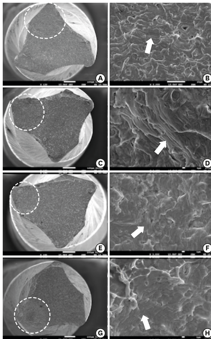
Figure 1. Scanning electron microscopic images of the WaveOne (WO) Primary files after cyclic fatigue testing. Views of the fractured surface in (A) the 0 WO group; (C) the 1 WO group; (E) the PF + WO group; (G) the PG + WO group, and high magnification views of (B) the 0 WO group; (D) the 1 WO group; (F) the PF + WO group; and (H) the PG + WO group showing typical fatigue striations indicative of cyclic fatigue. PF, PathFile; PG, ProGlider.
