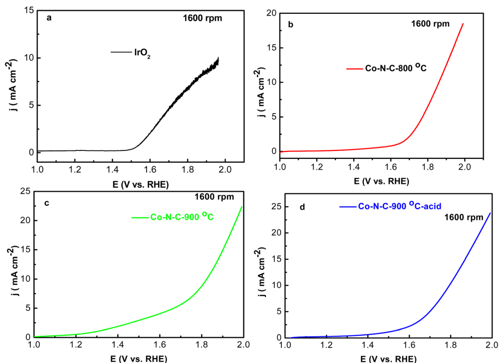
Fig. 6 Linear sweep voltammetry (LSV) of \text{IrO}_2 (a), Co-N-C-800 (b), Co-N-C-900 (c) and Co-N-C-900-acid (d) catalysts for oxygen evolution in \text{O}_2 -saturated 0.1 M KOH at various rotation speeds and scan rate of 5 \text{ mV s}^{-1} with 1600 rpm rotation rate.
