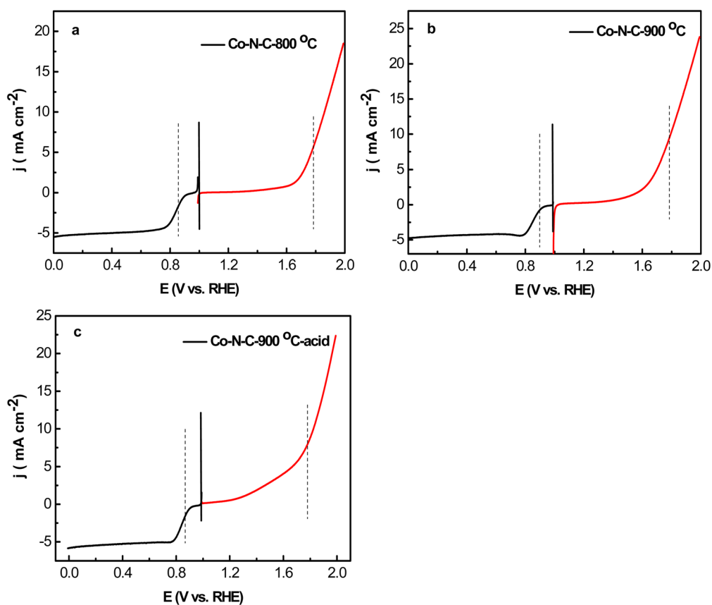
Fig. 7 ORR and OER potential difference curves of Co-N-C-800 (a), Co-N-C-900 (b) and Co-N-C-900-acid (c) catalysts in \text{O}_2 -saturated 0.1 M KOH with 1600 rpm and scan rate of 5 \text{ mV s}^{-1} .
