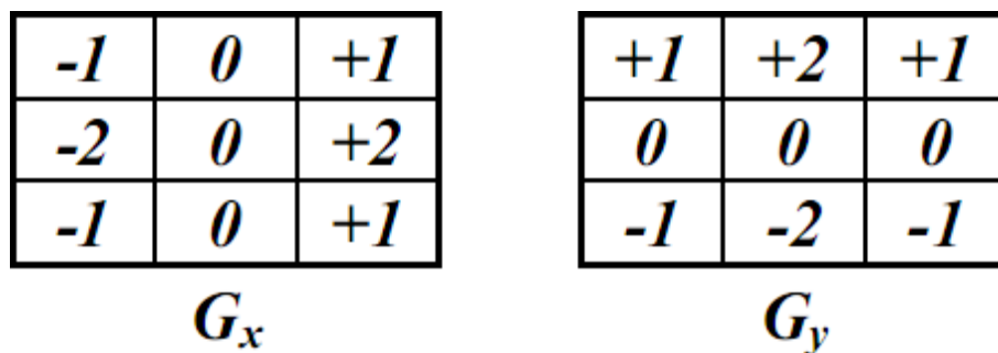
Figure 9 Two convolution masks of Sobel operator.
