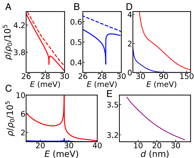
Fig. 4. Purcell factor near a vacuum-hBN-graphene-hBN-superconductor heterostructure. In A and B the graphene Fermi energy has been set at E_F^{gr} = 0.25 eV; here, T = 1 K for the solid curves and T = 94 K (above T_c ) for the dashed curves, and the graphene sheet is placed 4 nm above the superconductor surface. We show results for two emitter-graphene distances: 13 nm (A) and 36 nm (B). In C we show the case without graphene, at T = 1 K. The red curve corresponds to an emitter-superconductor separation of 17 nm and the blue curve to that of 40 nm. In D we show results for the same distances as in A (red curve) and B (blue curve), but for T = 94 K. In E we show how the Purcell factor depends on the graphene-superconductor distance t at the energy of the Higgs mode, \hbar\omega_H = 2\Delta_0 \approx 28.32 meV. The other parameters are kept fixed: E_F^{gr} = 0.5 eV, T = 1 K, and emitter-graphene distance of d = 13 nm. Here, graphene's conductivity has been modeled using the nonlocal random-phase approximation (23, 60).
