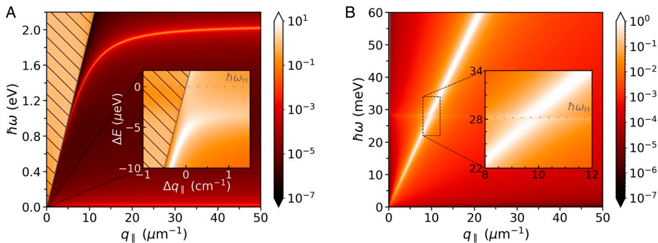
Fig. 2. Spectra of surface electromagnetic waves in superconductors (A) and graphene–superconductor (B) structures, obtained from the calculation of the corresponding \text{Im} r_p . (A) Dispersion diagram of SPPs supported by a vacuum–superconductor interface (the hatched area indicates the light cone in vacuum). Inset shows a closeup of an extremely small region (notice the change of scale) where the SPP dispersion crosses the energy associated with the superconductor’s Higgs mode; here, \Delta E = E - \hbar\omega_H and \Delta q_{\parallel} = q_{\parallel} - \omega_H/c . (B) Dispersion relation of GPs exhibiting an anticrossing feature that signals their interaction with the Higgs mode of the nearby superconductor. The graphene–superconductor separation is t = 5 nm. Setup parameters: We take T = 1 K; moreover, n = 6 \times 10^{21} \text{ cm}^{-3} (so that E_F \approx 1.20 eV and \hbar\omega_p \approx 2.88 eV), \hbar\gamma = 1 \mu\text{eV} , and T_c = 93 K for the superconductor (38, 40, 41), and E_F^{\text{gr}} = 0.3 eV and \hbar\gamma^{\text{gr}} = 1 meV, for graphene’s Drude-like optical conductivity (43).
