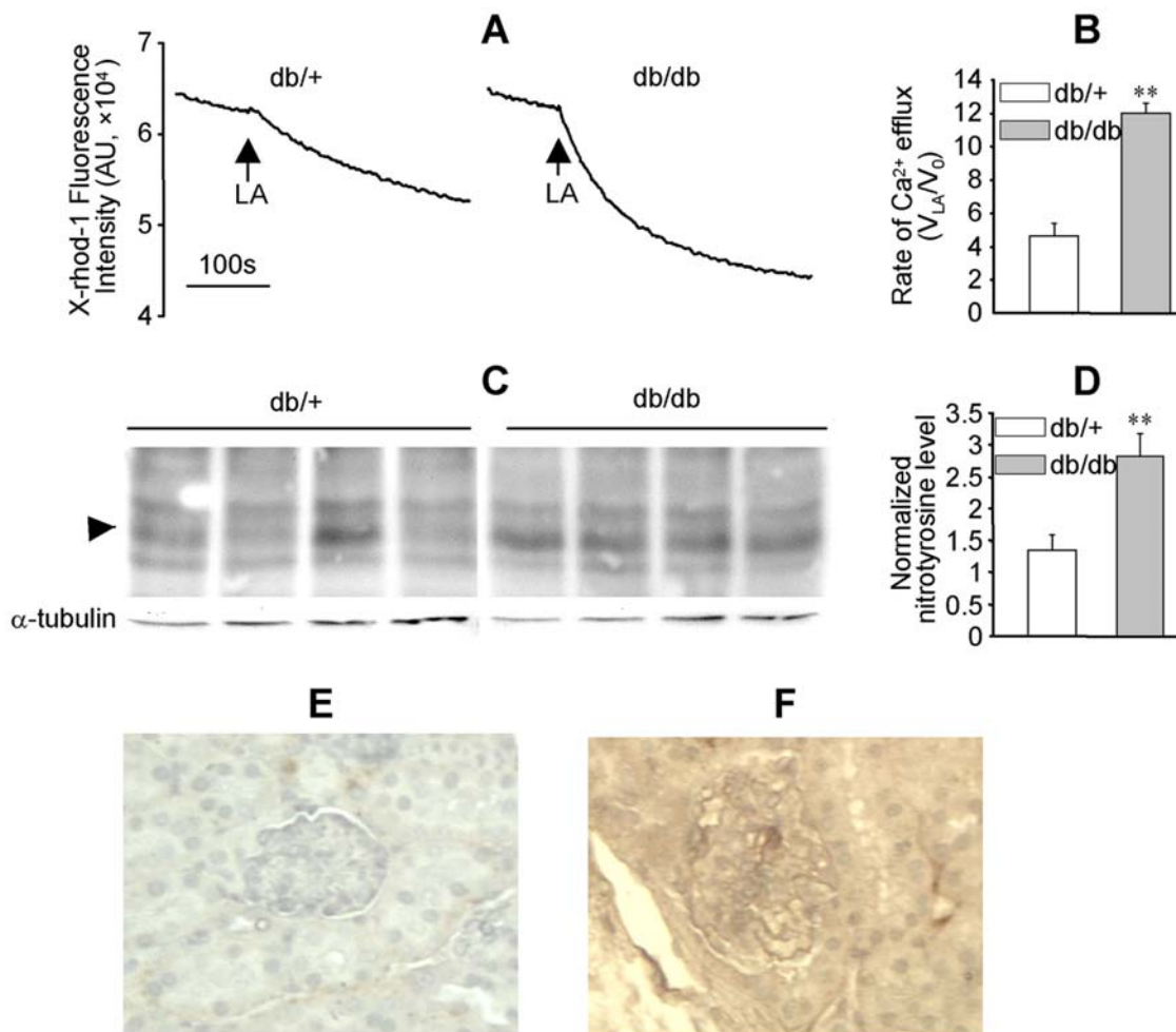
Figure 7. LA-induced mitochondrial Ca 2+ efflux and protein nitrotyrosylation were enhanced in the kidney of db/db mice. Mitochondria were prepared from fresh kidney tissues of 12–16 wk old db/+ and db/db mice and labeled with X-rhod-1 (2 \mu M). (A): LA-induced mitochondrial Ca 2+ efflux in the kidney of db/+ and db/db mice. (B): The ratio of the initial rate of LA-induced mitochondrial Ca 2+ efflux (V LA ; measured in the first 60 s following LA) to the basal rate (V 0 ; measured prior to LA). The values represent mean \pm SEM of V LA /V 0 , **P<0.01, n=3. (C) and (D): Nitrotyrosine levels in the kidney homogenates of four pairs of db/+ and db/db mice were analyzed by western blot using \alpha -tubulin as loading control. The arrowhead highlights a protein band (~22 kDa) with enhanced nitrotyrosine levels in db/db mice, **P<0.01, n=4. (E) and (F): Representatives of the nitrotyrosine levels in the kidney sections of db/+ and db/db mice as determined by immunohistochemistry. doi:10.1371/journal.pone.0006048.g007
