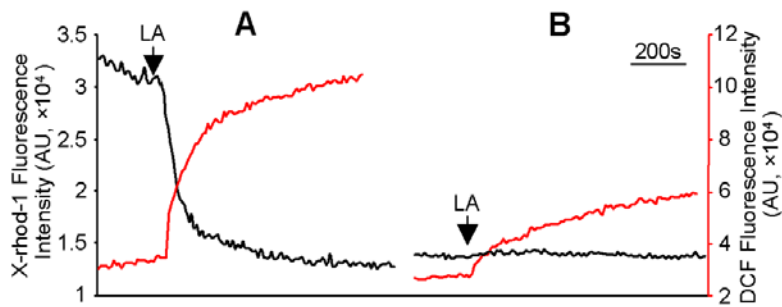
Figure 4. LA-induced mitochondrial Ca 2+ efflux was responsible for peroxynitrite generation. Mitochondria were prepared from HM cells and labeled with X-rhod-1 (2 μM) and DCF (1 μM) with (A) or without Ca 2+ (B). LA-induced mitochondrial Ca 2+ efflux (black traces) and peroxynitrite generation (red traces) were indexed by the gradual decrease in X-rhod-1 and increase in DCF fluorescence intensity, respectively. doi:10.1371/journal.pone.0006048.g004
