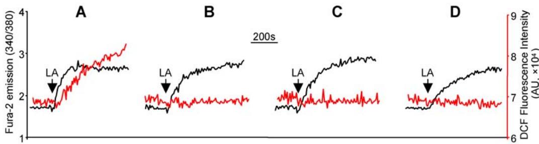
Figure 6. Mitochondrial complexes I and III were required for LA-induced peroxynitrite generation. HM cells were labeled with fura-2 and DCF to measure LA responsive [Ca 2+ ] m mobilization (black traces) and peroxynitrite generation (red traces). (A): LA responses in untreated cells (control); (B) LA responses in cells pretreated with rotenone (a mitochondrial complex I inhibitor, 10 μM, 20 min); (C) and (D): LA responses in cells pretreated with the mitochondrial complex III blockers, antimycin A (1 μM, 20 min); C) or myxothiazol (0.5 μM, 60 min); D). doi:10.1371/journal.pone.0006048.g006
