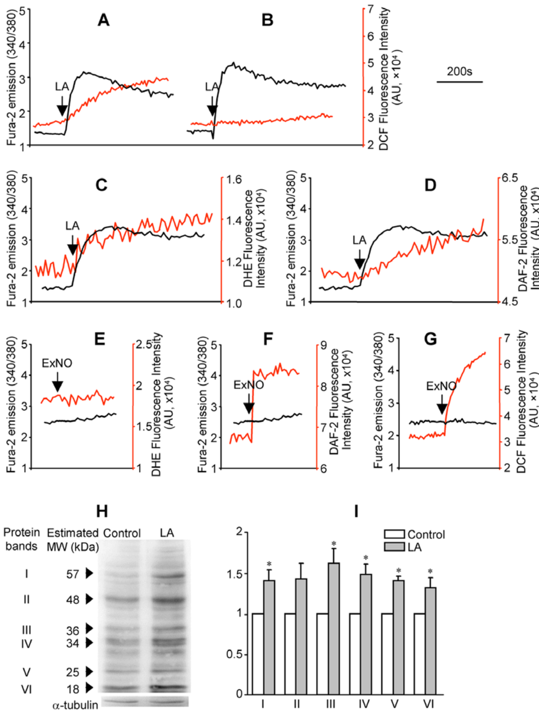
Figure 2. The LA-induced ROS signal was identified as peroxynitrite. (A): HM cells were labeled with fura-2 and DCF and traces represent LA-induced [Ca^{2+}]_i mobilization (black trace) and ROS generation (red trace); (B): same measurements performed in cells treated with FeTPPS (a specific peroxynitrite decomposer; 0.5 \mu M, 30 min) prior to LA addition and the treatment inhibited the ROS signal significantly; (C) and (E): HM cells were labeled with fura-2 and dihydroethidium (DHE, 1 \mu M) and traces represent LA (C) or S-nitroso-N-acetylpenicillamine (exogenous NO donor, ExNO, 50 \mu M; E) responsive [Ca^{2+}]_i mobilization (black trace) and superoxide generation (red trace); (D) and (F): HM cells were labeled with fura-2 and 4,5-diaminofluorescein diacetate (DAF-2, 0.5 nM) and traces represent LA (D) or ExNO (F) responsive [Ca^{2+}]_i mobilization (black trace) and NO generation (red trace); (G) HM cells were labeled with fura-2 and DCF and traces represent ExNO responses in [Ca^{2+}]_i (black trace) and peroxynitrite (red trace). The nitrotyrosine level in the cellular proteins was determined by western blot analysis in vehicle-(control) or LA-treated HM cells using \alpha -tubulin as the loading control. The image (H) shows a representative experiment. The graphs (I) represent the mean ratio value \pm SEM of the density of protein band over \alpha -tubulin. * P <0.05, n =4, LA vs control. doi:10.1371/journal.pone.0006048.g002
