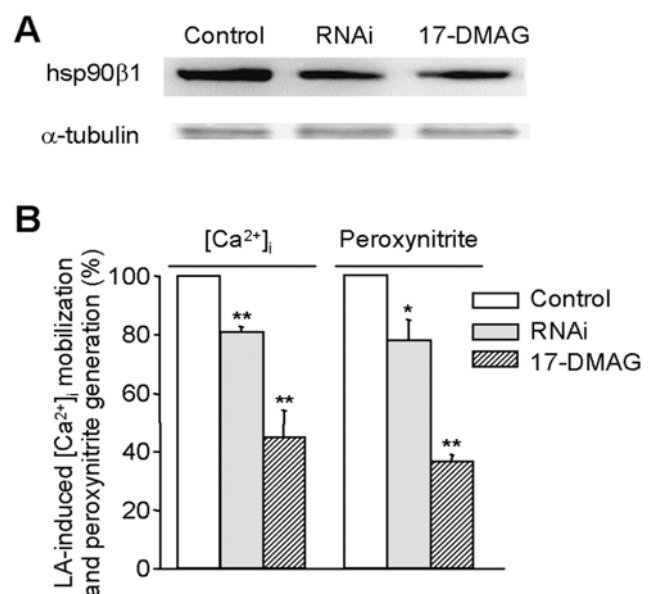
Figure 5. The effect of hsp90β1 on LA-induced [Ca 2+ ] i mobilization and peroxynitrite generation. HM cells were treated with vehicle (control), hsp90β1 RNAi, or 17-DMAG for 48 h. (A): Cell lysates were prepared and the alterations of hsp90β1 expression were analyzed by western blot analysis using α-tubulin as loading control. (B): The alteration of LA-induced [Ca 2+ ] i mobilization and peroxynitrite generation in hsp90β1 RNAi- and 17-DMAG-treated HM cells relative to control. The values represent the mean ± SEM. * P <0.05, ** P <0.01, n =6. doi:10.1371/journal.pone.0006048.g005
