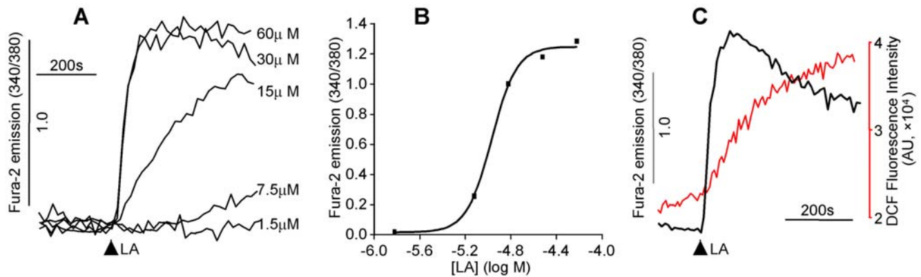
Figure 1. LA-induced [Ca 2+ ] i mobilization and ROS generation. Human mesangial cells were labeled with fura-2 (1 μM) alone or together with DCF (1 μM) (37°C, 30 min). The fluorescent intensity in the figures was presented as arbitrary unit (AU). (A): Traces represent the [Ca 2+ ] i responses induced by different concentrations of LA. (B): The curve shows the relationship between the amplitude of [Ca 2+ ] i responses and the LA concentrations. (C): Traces represent LA (30 μM)-induced [Ca 2+ ] i mobilization (black trace) and the associated ROS generation (red trace). doi:10.1371/journal.pone.0006048.g001
