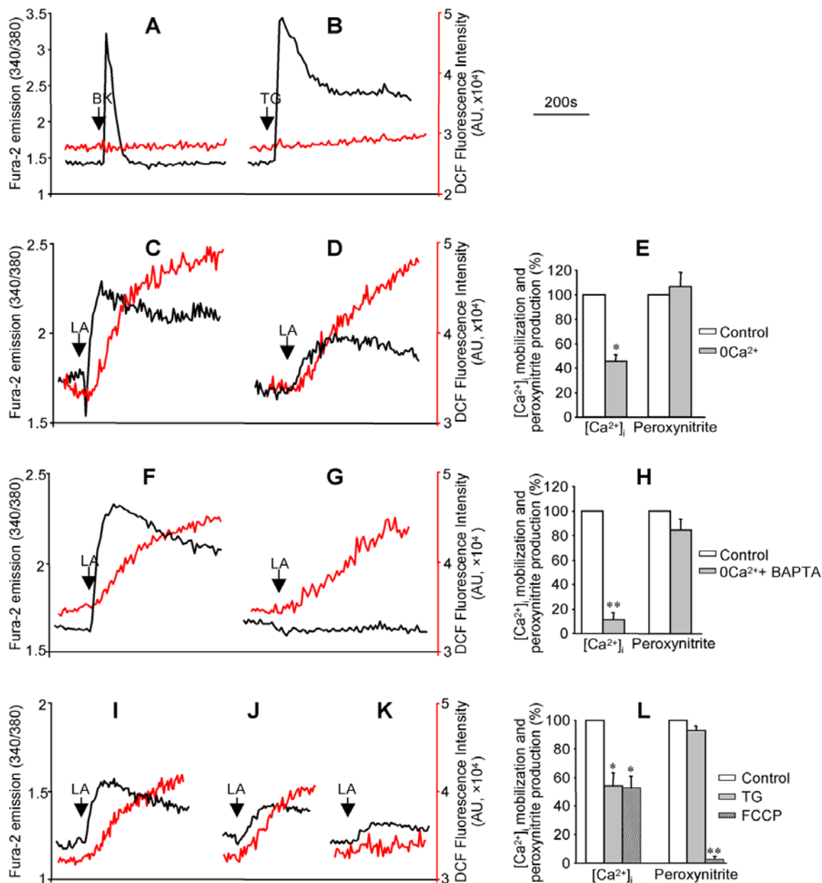
Figure 3. Mitochondria played an essential role in LA-induced [Ca 2+ ] i mobilization and peroxynitrite generation. HM cells were labeled with fura-2 and DCF to measure [Ca 2+ ] i mobilization (black traces) and peroxynitrite generation (red traces). (A): Bradykinin (BK, 100 nM) responses; (B): thapsigargin (TG, 2 μM) responses; (C) and (F): LA responses measured in the presence of extracellular Ca 2+ (control); (D): LA responses measured without extracellular Ca 2+ ; (G) LA responses measured in cells pretreated with BAPTA (50 μM, 30 min) without extracellular Ca 2+ . In the absence of extracellular Ca 2+ , (I): LA responses (control); (J): LA responses in cells pretreated with TG (2 μM, 5 min); (K) LA responses in cells pretreated with FCCP (a mitochondrial uncoupler; 4 μM, 5 min). The values in graphs (E, H, and L) represent the mean ± SEM of the relative amplitudes of LA-induced [Ca 2+ ] i and peroxynitrite responses, * P < 0.05, ** P < 0.01, n = 6, treated cells vs control. doi:10.1371/journal.pone.0006048.g003
