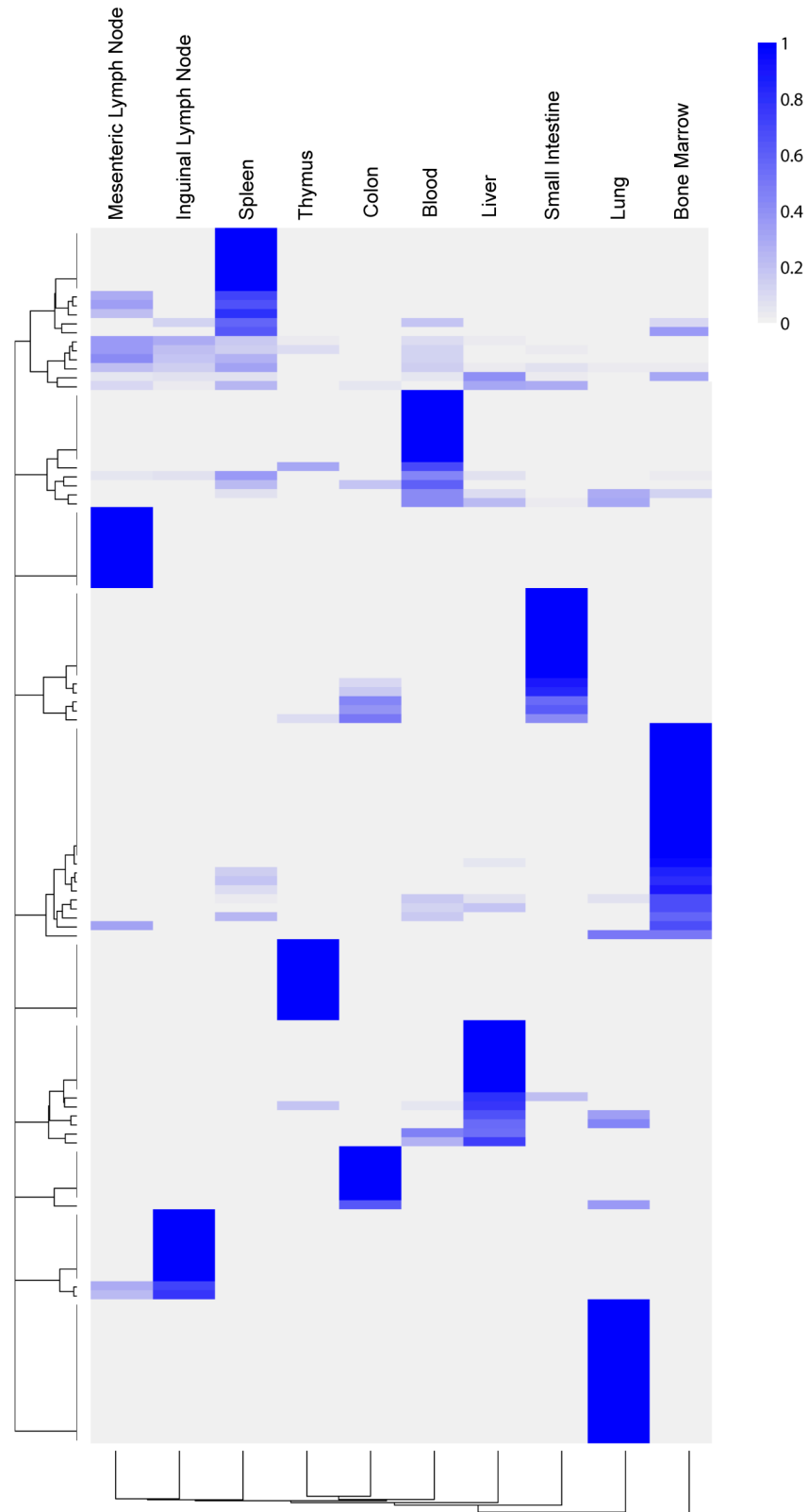
Fig 14. Heatmap of clade proportions across the tissue samples. Sample-specific clades have a value of 1, while shared clades have proportions spread across different samples. Physiologically similar samples share more clades. S13 Fig is a higher resolution version of Fig 14 with clade labels.
