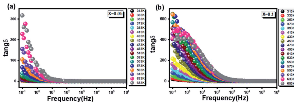
Fig. 10 The frequency dependence at different temperatures of the loss factor for the two \text{Ag}_x\text{Zn}_{1-x}\text{Al}_2\text{O}_4 ( x = 0.05 (a) and x = 0.1 (b)) samples.
