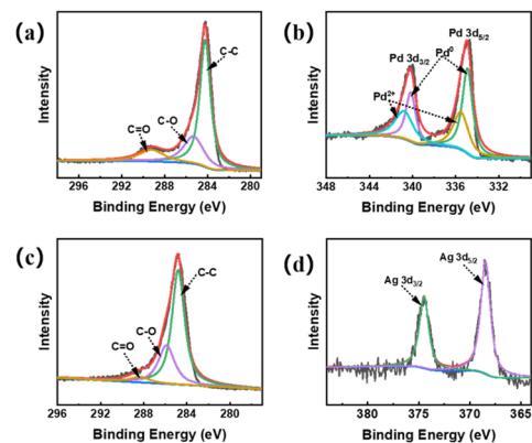
Fig. 3 XPS profiles of Pd/p-C nanocomposites: (a) C 1s; (b) Pd 3d; XPS profiles of Ag/p-C nanocomposites: (c) C 1s; (d) Ag 3d.
