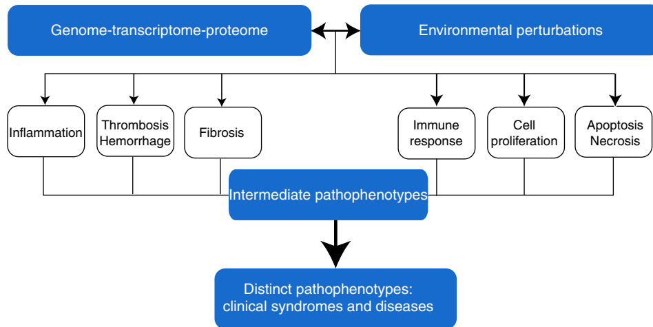
Figure 1 Diagram indicating associations among genetic and environmental factors reduce and their interactions with intermediate phenotypes to yield distinct pathophenotypes. The intermediate phenotypes determine, in part, variation in disease expression and clinical presentation among individuals with equivalent underlying genetic or environmental exposures that predispose to a disease state.
