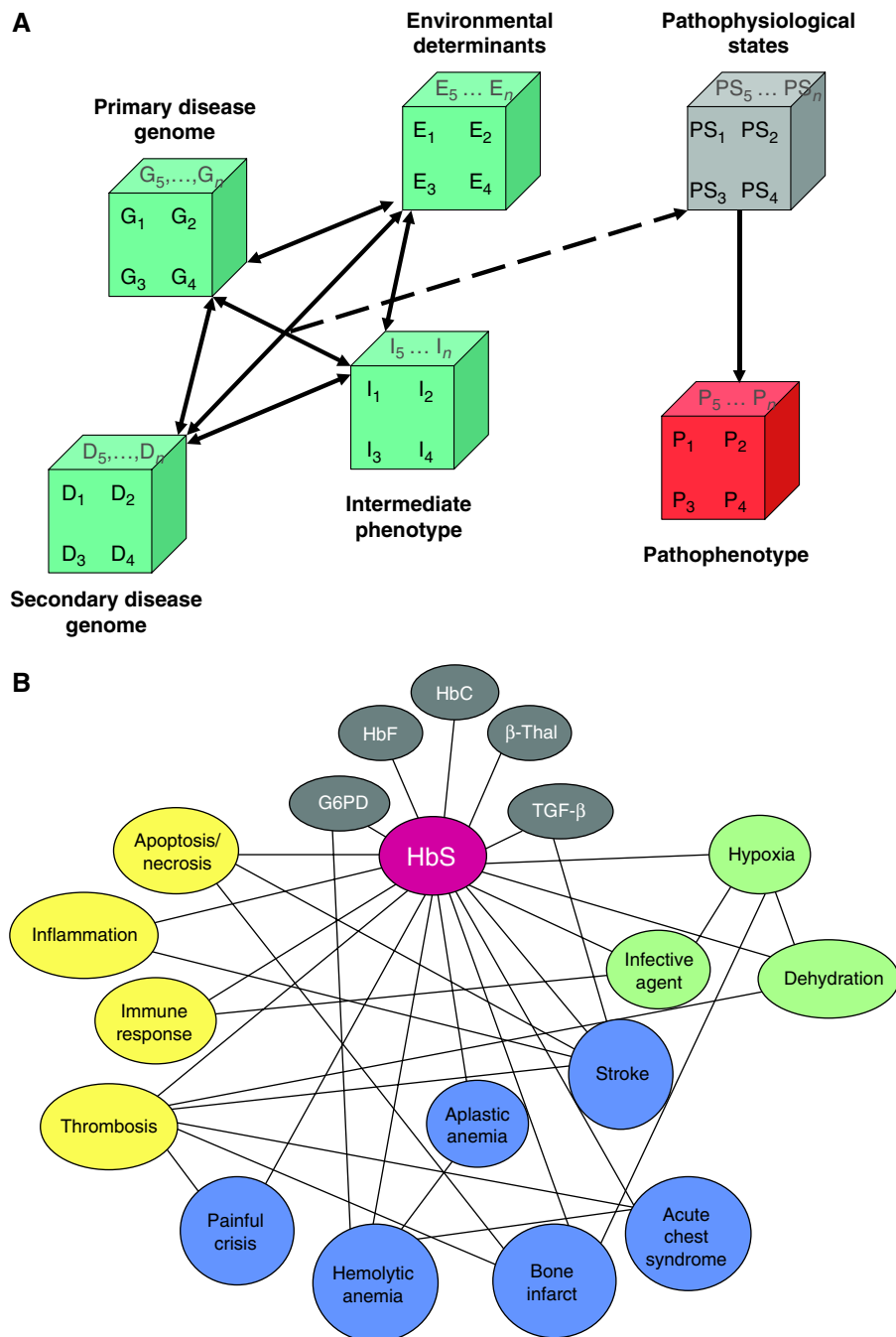
Figure 2 (A) Theoretical human disease network illustrating the relationships among genetic and environmental determinants of the pathophenotypes. Key: G, primary disease genome or proteome; D, secondary disease genome or proteome; I, intermediate phenotype; E, environmental determinants; PS, pathophysiological states leading to P, pathophenotype. (B) Example of this theoretical construct applied to sickle cell disease. Key: red, primary molecular abnormality; gray, disease-modifying genes; yellow, intermediate phenotypes; green, environmental determinants; blue, pathophenotypes.
