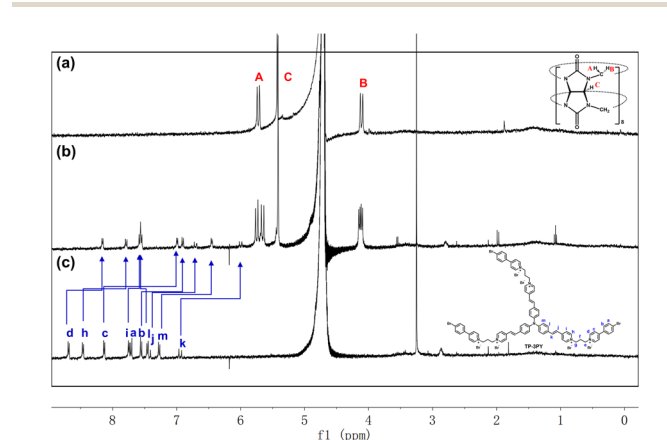
Fig. 1 1 H NMR spectra of (a) CB[8], (b) TP-3PY⊂CB[8] and (c) TP-3PY ([TP-3PY] = 3 \times 10^{-4} \text{ M} , [CB[8]] = 9 \times 10^{-4} \text{ M} , 400 MHz, D 2 O, 298 K).
