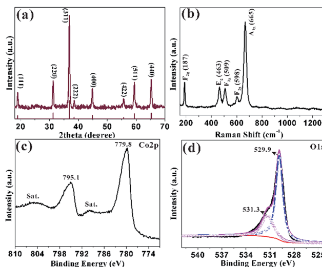
Fig. 2 (a) XRD pattern of the sample obtained at 300 \text{ }^\circ\text{C} for 1 h; (b) the corresponding Raman spectrum; XPS spectra of (c) Co 2p; (d) O 1s.
