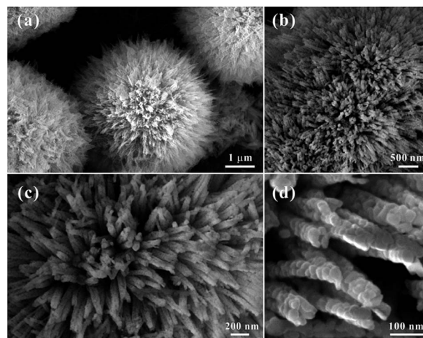
Fig. 1 FE-SEM images of the 3D hierarchical \text{Co}_3\text{O}_4 microspheres (HCMs) with porous nanorods building units obtained by calcination precursor at 300 \text{ }^\circ\text{C} for 1 h. (a) Overall product morphology; (b and c) detailed view of an individual hierarchitecte; (d) magnified image of the nanorods structure of the hierarchitecte.
