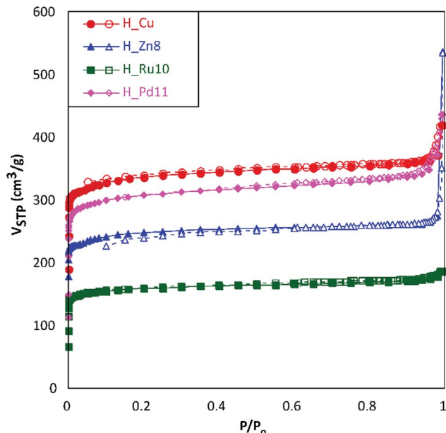
Fig. 4 N 2 adsorption isotherms at 77 K for H_Cu, H_Zn8, H_Ru10 and H_Pd11. Filled and empty symbols correspond to adsorption and desorption branches, respectively.
