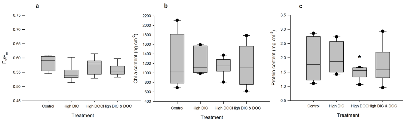
Fig 5. Photosystem parameters as response to treatments. Maximum quantum yield (a) of dark adapted individuals of Acropora millepora (Ehrenberg, 1834) (n = 12). Chlorophyll content (b) related to fresh weight (n = 6). Protein content (c) of A. millepora related to surface area (n = 6). Data are compared between the control, the high DIC treatment ( p\text{CO}_2 403 \mu\text{atm} ), the high DOC treatment (DOC (added as Glucose 0 and 294 \mu\text{mol L}^{-1} ) and the combination of both treatments. Boxplots indicating median (mid of boxplot), 25% and 75% percentile (lower and upper border of boxplot) and 90 and 10% percentile (whiskers). Significant differences ( p < 0.05 ) are marked with an asterisk
