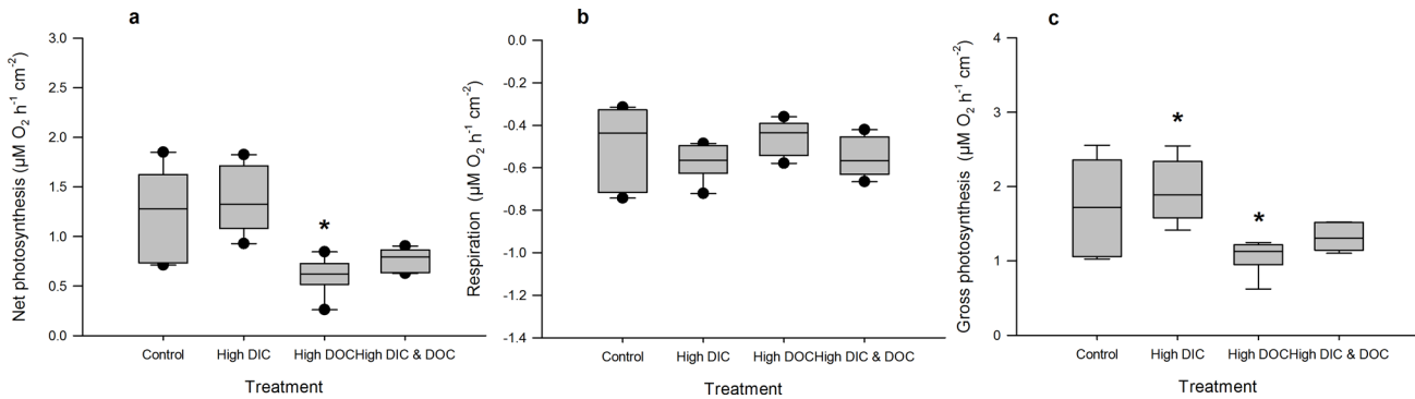
Fig 4. Oxygen fluxes as responses to treatments. Net photosynthesis (a), respiration (b) and gross photosynthesis (c) of Acropora millepora (Ehrenberg, 1834) (n = 6). Net photosynthesis measured during light ( 150 \mu \text{ photons} \cdot \text{m}^{-2} \cdot \text{s}^{-1} ) conditions and respiration during dark condition and related to coral surface area. Data are compared between the control, the high DIC treatment ( p\text{CO}_2 403 \mu\text{atm} ), the high DOC treatment (DOC (added as Glucose 0 and 294 \mu\text{mol L}^{-1} ) and the combination of both treatments. Boxplots indicating median (mid of boxplot), 25% and 75% percentile (lower and upper border of boxplot) and 90 and 10% percentile (whiskers). Significant differences ( p < 0.05 ) are marked with an asterisk
