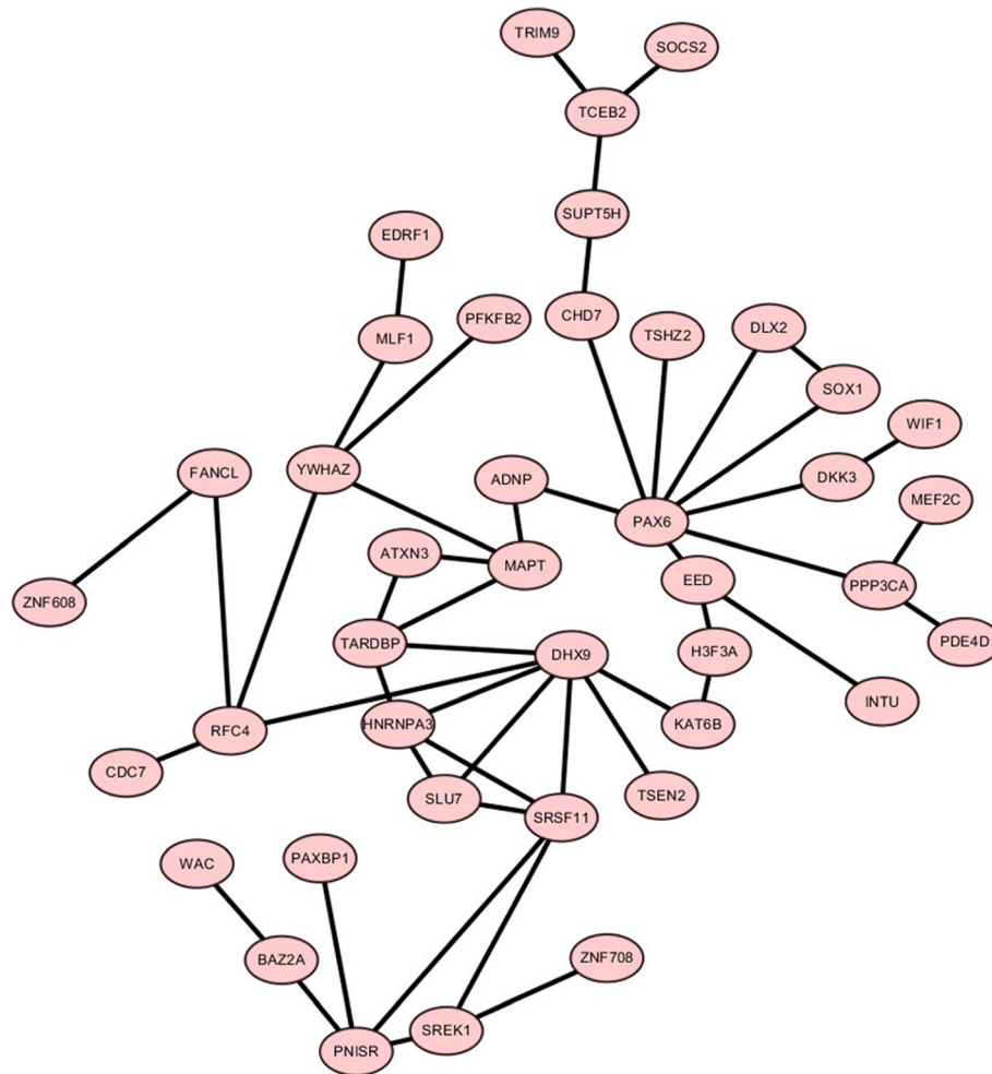
Fig. 5 The subgroup protein–protein interaction (PPI) analysis of the hypermethylation-low expression genes (Hyper-LGs)
