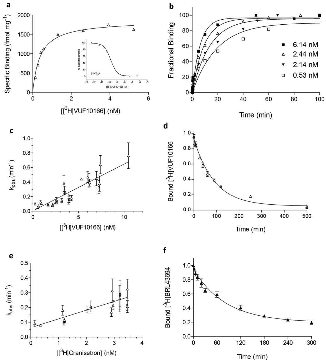
Fig. 1. Radioligand binding at 5-HT 3 A receptors. (a) Representative binding curves for 5-HT 3 A receptors. Inset competition binding of unlabelled VUF10166 with [³H]granisetron. (b) Association of [³H]VUF10166 was fit with a mono-exponential function to yield k_{obs} . (c) Linear regression was used to fit k_{obs} against the radioligand concentration, yielding the k_{on} (slope) and k_{off} (intercept at y = 0 ) values in Table 1. (d) Dissociation of [³H]VUF10166 was best fit with a single exponential ( k_{off} = 0.011 \pm 0.001 \text{ min}^{-1} , n = 4 ). (e) For [³H]granisetron, association was also best fit with mono-exponential functions that were used to plot k_{obs} against the concentration to yield the k_{on} and k_{off} values in Table 1. (f) Dissociation of [³H]granisetron ( k_{off} = 0.011 \pm 0.001 \text{ min}^{-1} , n = 5 ).
