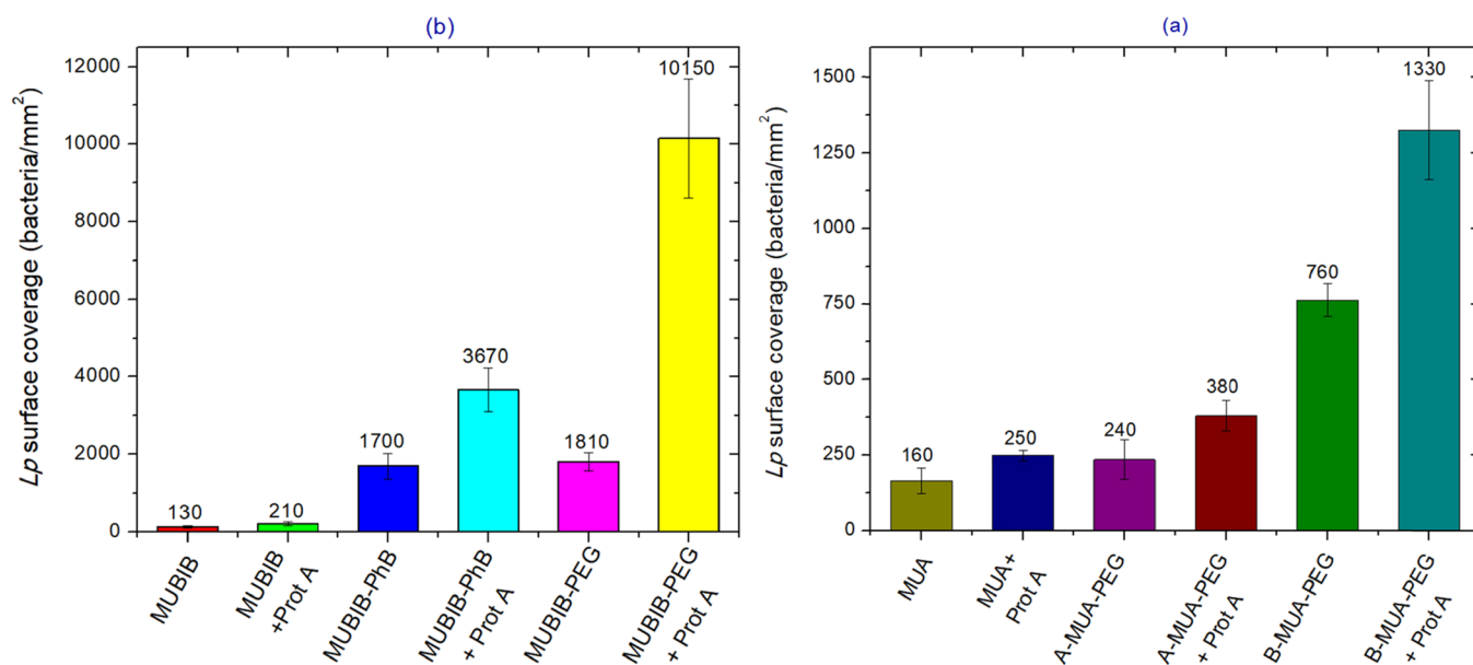
Figure 5. Surface coverage of captured GFP Lp on the surface of (a) MUA SAM- and MUA-based PB-coated GaAs samples and (b) MUBIB SAM- and MUBIB-based PB-coated GaAs samples, with and without protein A.
