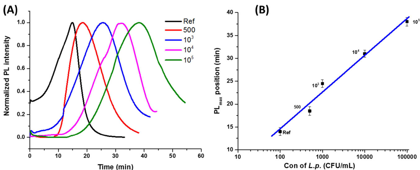
Figure 6. Representative temporal PL intensity plots of GaAs/AlGaAs polymer brush (MUBIB-PEG)-functionalized biochips digitally photocorroding (Duty Cycle = 1.5/11) under continuous flow of 0.1\times PBS and different concentrations of bacteria (A). Calibration curve based on the position of the PL intensity maximum revealed with the digital photocorrosion process for the GaAs (12 nm)/AlGaAs (10 nm) nanoheterostructure (B).
