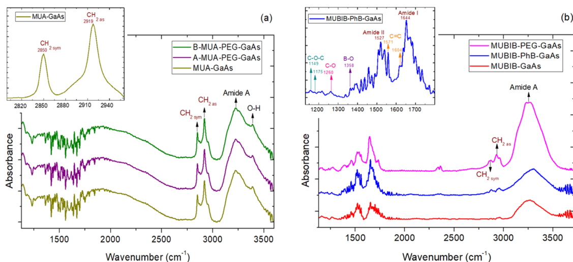
Figure 2. FTIR absorbance spectra of anti- Lp antibodies immobilized on (a) MUA SAM- and MUA-based PB-coated GaAs samples and (b) MUBIB SAM- and MUBIB-based PB-coated GaAs samples. Each spectrum represents an example of one of three tested samples.
