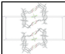
Fig. 2. Part of the crystal packing of the title compound, viewed along the c axis, showing dimers stacked along the c axis. Hydrogen bonds are shown as dashed lines. For clarity, Only two disorder components of the chloroform solvent molecule are shown.
