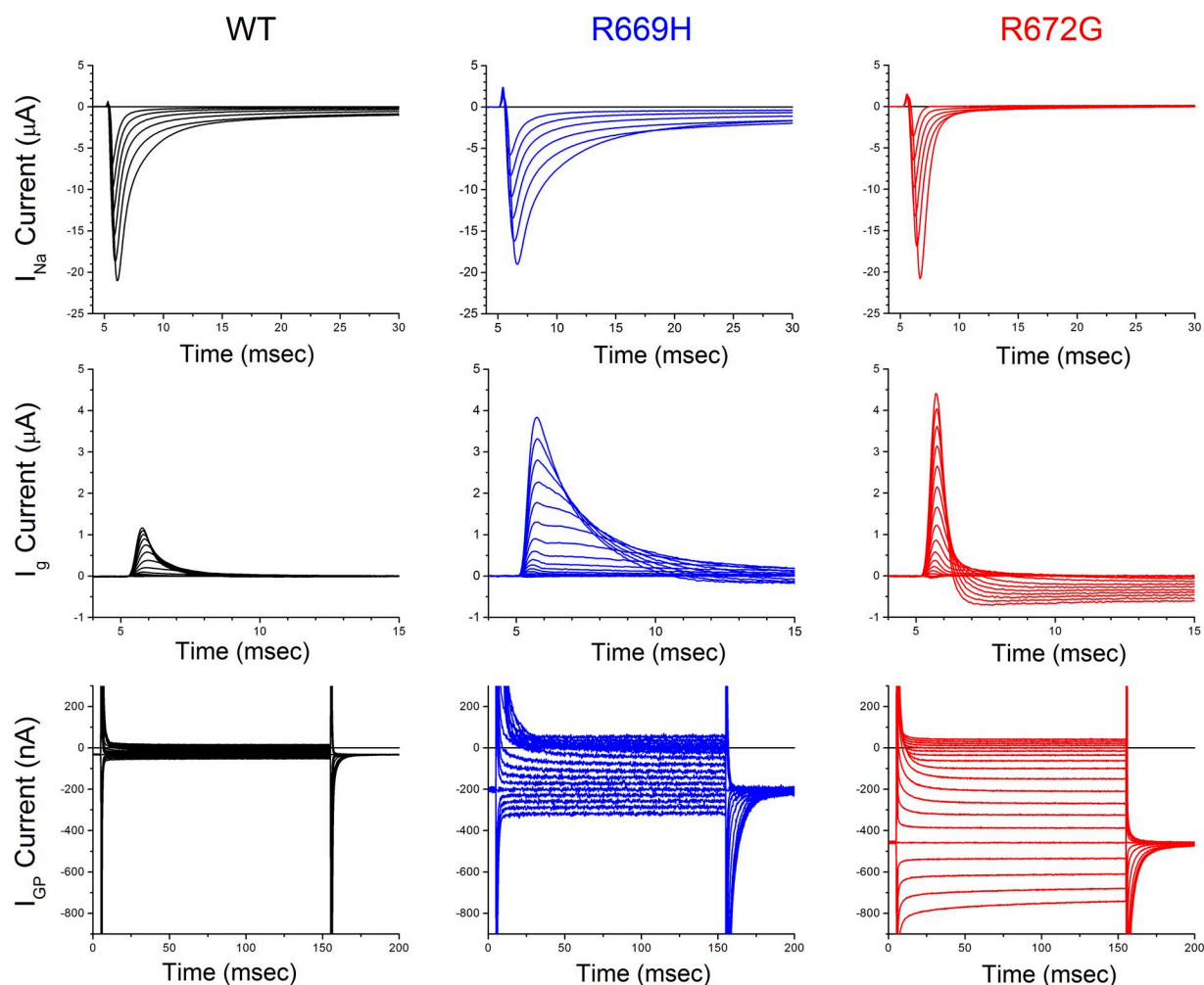
Figure 1. Currents, recorded under different conditions for the same oocyte, to measure I_{\text{Na}} , I_{\text{g}} , and I_{\text{GP}} . First, \text{Na}^+ currents were recorded in a 115-mM \text{Na}^+ bath with analogue compensation for linear capacitance and digital P/N subtraction of residual linear leak (top row). Responses are shown for test potentials of -20 to 30 mV. The external solution was then exchanged with \text{K}^+ /TTX (R672G) or NMDG ^+ /TTX (R669H or WT), and P/N leak subtraction was performed to reveal the nonlinear gating charge displacement current, I_{\text{g}} (middle row). Finally, all analogue and digital P/N leak subtraction was omitted to reveal the gating pore current for mutant channels and the residual leakage current for oocytes expressing WT channels (bottom row). Each column shows the responses recorded from a single oocyte (black, WT; blue, R669H; red, R672G).
