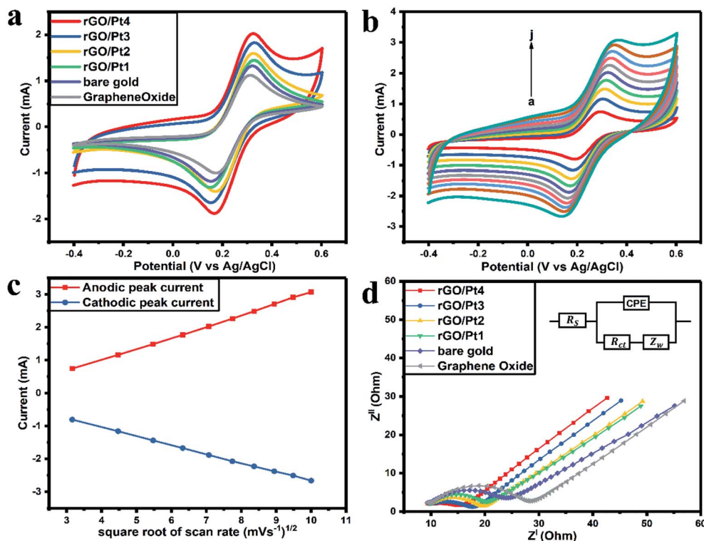
Fig. 6 (a) Cyclic voltammograms of GO, bare gold, rGO/Pt1, rGO/Pt2, rGO/Pt3 and rGO/Pt4-modified gold electrodes in the presence of 5 mM [Fe(CN) 6 ] -3/-4 in 0.5 M PBS (pH 7.4, 0.15 M NaCl). (b) Cyclic voltammograms of the rGO/Pt4-modified gold electrode with various scan rates from 10 to 100 mV s -1 (a–j). (c) Variations of I_a and I_c with changes in the square root of the scan rate for rGO/Pt4. (d) The Nyquist plots of the GO, bare gold and rGO/Pt nanocomposite electrodes (inset shows the Randles equivalent circuit).
