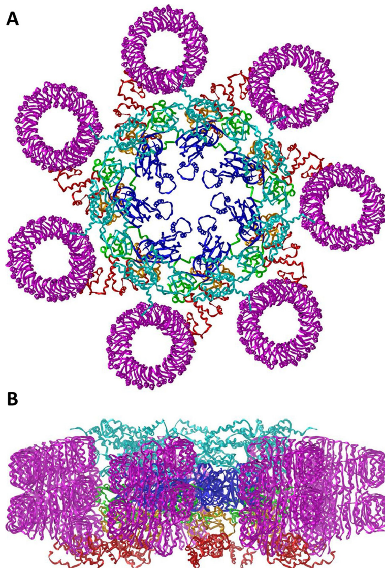
Figure 7 A model for heptameric full-length human NLRC5. Top (A) and side views (B) are represented. Domain and color codes: uCARD: cyan, NACHT: blue, AxP: green, WH: orange, SH: red, LRR: magenta.
