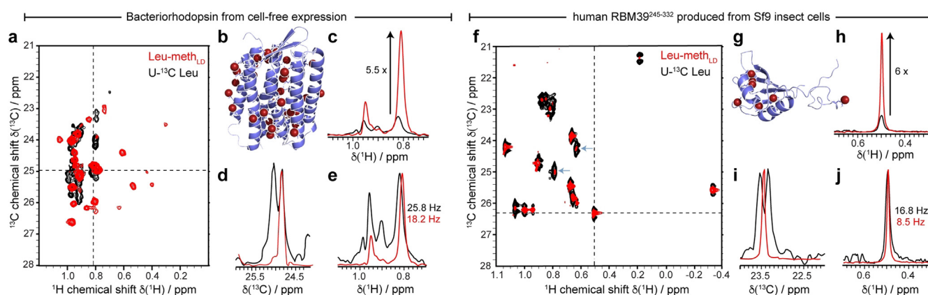
Figure 3. Stereo-specific \text{CD}_3/^{13}\text{CH}_3 -labeled Leu with Leu-meth LD facilitates NMR characterization of proteins expressed in vitro and in insect cells. (a) ^{13}\text{C} , ^1\text{H} -HSQC spectra of cell-free expressed bR in DDM micelles with [\text{U-}^{13}\text{C}, ^1\text{H}] Leu (black) or Leu-meth LD (red). (b) Structure of bacteriorhodopsin (bR, PDB ID:1R84) with ^{13}\text{C} , ^1\text{H} -labeled Leu methyl groups highlighted as red spheres. One-dimensional slices at indicated frequency in the ^1\text{H}/^{13}\text{C} dimension are shown in (c)–(e). (c) Signal intensity is increased by 5.5-fold. Comparison of normalized data shows that a singlet is obtained instead of doublet facilitating high resolution acquisition in the ^{13}\text{C} dimension (d) and that linewidth at half-height is reduced by 29% in the ^1\text{H} dimension (e). (f) ^{13}\text{C} , ^1\text{H} -HSQC spectra of the human RBM39 245–332 encapsulating RRM2 domain expressed in insect cells with [\text{U-}^{13}\text{C}, ^1\text{H}] Leu (black) or Leu-meth LD (red). (g) Structure of the CAPER-RRM2 domain (PDB ID: 2JRS) with ^{13}\text{C} , ^1\text{H} labeled Leu methyl groups highlighted as red spheres. Some of the residual 6% of inverted methyl labeled leucines are also observable (example marked by a blue arrow). Analog as for bR (c–e), one-dimensional slices at indicated frequency in the ^1\text{H}/^{13}\text{C} dimension are shown in (h)–(j). (h) Signal intensity is increased by 6-fold. (j) Linewidth at half height is reduced by 49% in the ^1\text{H} dimension.
