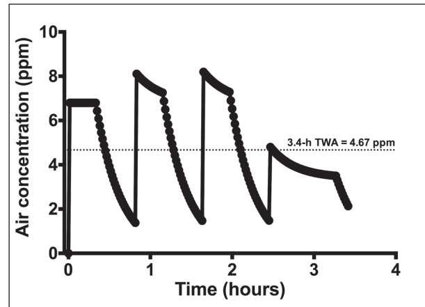
Figure 2. Modeled concentrations of sevoflurane in the air in the treatment room used for topical treatment. The usage rate of sevoflurane was close to 1 patient every 50 min, the volume of the room and the air changes used corresponded to the real scenario conditions (163 m 3 and 3.3 per hour, respectively). Each peak represents a new patient treated. The dotted line represents the ppm-TWA for the entire exposure period. The peak concentrations and the ppm-TWA remain under exposure limits set by occupational safety agencies from Finland, Sweden, and Norway.
