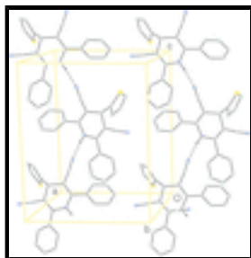
Fig. 2. A partial packing diagram. Hydrogen bonds are shown as dashed lines. Hydrogen atoms not involved in hydrogen bonding are omitted for clarity.
