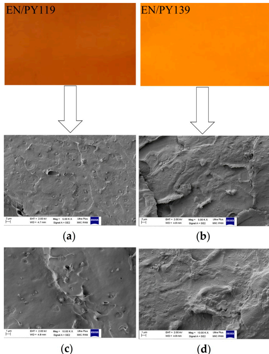
Figure 2. Digital photos and SEM images showing the EN copolymer containing PY119 (a,c) and PY139 (b,d) at different magnitudes.
