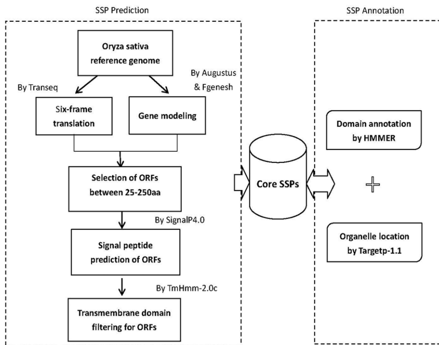
Figure 1. Schematic diagram of the data processing pipeline for OrysPSSP.
