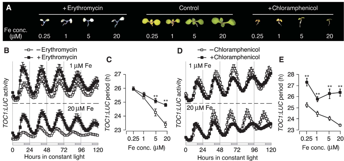
Figure 5 A block in chloroplast protein translation impairs circadian Fe responses. (A) Col-0 seedlings grown on Hoagland medium containing various Fe supply, alone or in combination with 50 \mu\text{M} erythromycin or 10 \mu\text{g/ml} chloramphenicol. (B, C) Circadian period length in seedlings treated with the plastid-specific protein translation inhibitor erythromycin responds less to Fe sufficiency. TOC1:LUC activity (B) and period lengths (C) in Col-2 seedlings grown on Hoagland medium containing various Fe supply and 50 \mu\text{M} erythromycin. (D, E) The plastid and mitochondria protein translation inhibitor chloramphenicol abolishes circadian Fe responses and results in a constitutive long period. TOC1:LUC activity (D) and period lengths (E) in Col-2 seedlings grown on Hoagland medium containing various Fe supply and 10 \mu\text{g/ml} chloramphenicol. **Significantly different between control and treated seedlings (two-tailed Student's t -test, P \leq 0.02 ).
