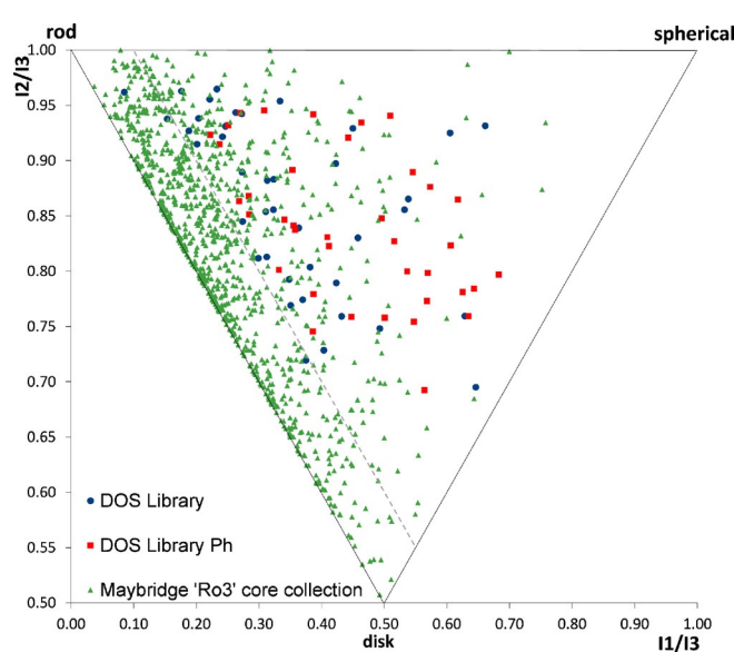
Figure 4. Comparative PMI plot analysis of DOS library (blue circles), Maybridge core 1000-member “Ro3” Fragment library (green triangles) and the DOS Ph virtual library (red squares). Compounds within “flatland” (represented by npr1 + npr2 < 1.1 , dashed line) could also be identified; the further from this area the molecules move the more they extend into three-dimensional space. [36]
