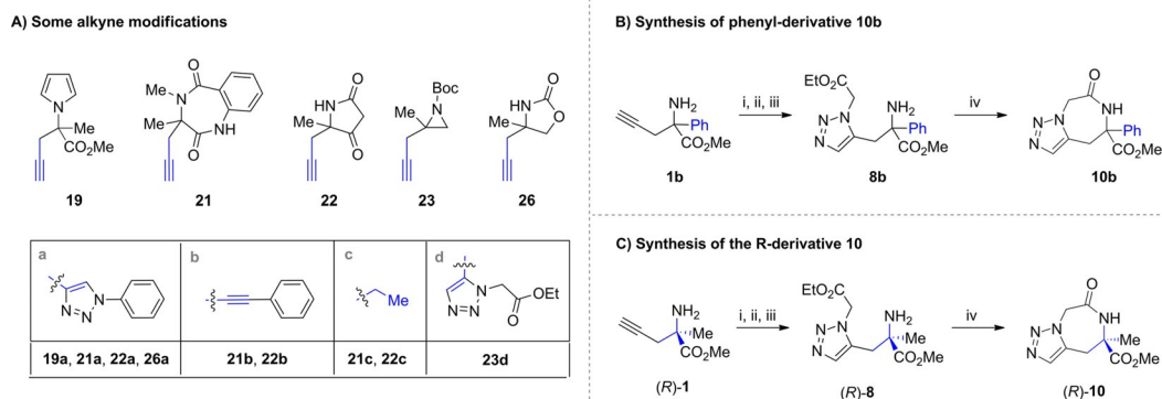
Figure 3. (A) Exemplification of the synthesis of other derivatives via alkyne modifications. Reaction conditions: 19 a , 21 a , 22 a , 26 a : azidobenzene, \text{CuSO}_4 \cdot 5\text{H}_2\text{O} , t\text{BuOH}:\text{H}_2\text{O} , rt, 72–92%; 21 b and 22 b : \text{PdCl}_2(\text{PPh}_3)_2 , \text{CuI} , \text{Et}_3\text{N} , benzyl 2-iodobenzoate, DMF, rt, 16 h, 60% and 26%, respectively; 21 c and 22 c : \text{Pd/C} , \text{H}_2 , MeOH, rt, 2 h, 69% and 87%, respectively; 23 d : ethyl 2-azidoacetate, \text{Cp}^*\text{RuCl}(\text{COD}) , PhMe, -60^\circ\text{C} , 21 h, 42% (B) Synthesis of the phenyl-containing derivative. Reaction conditions: i) \text{Boc}_2\text{O} , THF, 70^\circ\text{C} , o/n, 84%; ii) ethyl 2-azidoacetate, \text{Cp}^*\text{RuCl}(\text{COD}) , PhMe, 80^\circ\text{C} , 1 h, 87%; iii) TFA, \text{CH}_2\text{Cl}_2 , 2 h then \text{NaHCO}_3 , (quantitative yield); iv) PhMe, 150^\circ\text{C} , o/n, 76%. (C) Synthesis of an enantiopure component of the library. Reaction conditions: i) \text{Boc}_2\text{O} , THF, 70^\circ\text{C} , o/n, 90%; ii) ethyl 2-azidoacetate, \text{Cp}^*\text{RuCl}(\text{COD}) , PhMe, 50^\circ\text{C} , 1 h, 76%; iii) TFA, \text{CH}_2\text{Cl}_2 , 2 h then \text{NaHCO}_3 , 93%; iv) PhMe, 150^\circ\text{C} , o/n, 79%.
