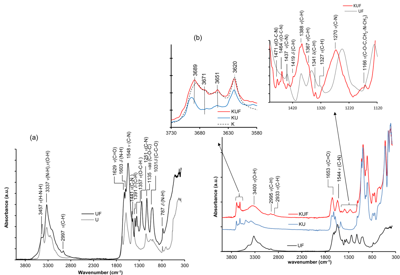
Fig. 5 FTIR spectra of (a) free poly(urea-formaldehyde) (UF) and urea (U); (b) urea-intercalated kaolinite (KU), and intercalated kaolinite-poly(urea-formaldehyde) (KUF). ν: Stretching vibrations; ν as : asymmetric stretching vibrations; δ: bending vibrations.
