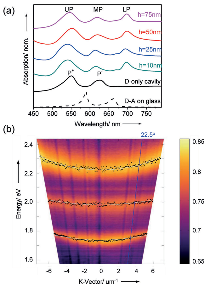
Figure 2. a) Normalized absorption spectra for various spacer thickness (10 nm to 75 nm) of donor (TDBC) and acceptor (BRK) in the strongly coupled cavity. The absorption A is determined after recording the transmission T and the reflection R of the samples ( A = 1 - T - R ). The black dash curve shows the spatial separated donor and acceptor absorbance spectrum on top of a glass substrate. b) Example of the reflection dispersion plots in the donor-acceptor ( h = 50 nm) strongly coupled cavity. The white lines correspond to the coupled oscillator model results with different Hopfield coefficient. The blue line indicates the angle ( 22.5^\circ ) where the excitation spectra were collected.
