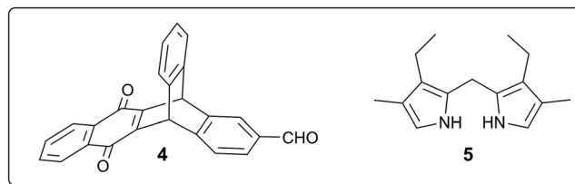
Scheme 2 (a) Reported synthetic route of TNQ-ZnP-TAPD using the protected TAPD precursor 3 . 7a,b (i) \text{BF}_3 \cdot \text{OEt}_2 , \text{DCM} then \text{DDQ} ; (ii) \text{SnCl}_2 , \text{HCl} ; (iii) \text{NaBH}_3\text{CN} , \text{CH}_2\text{O} ; (iv) \text{Zn}(\text{OAc})_2 , \text{CHCl}_3/\text{MeOH} ; (b) new synthesis of 3 . (v) \text{AcOH} , 12 h, 118 °C, 95%; (vi) \text{BH}_3 \cdot \text{THF} , \text{THF} , 12 h, 66 °C, 75%; (vii) activated \text{MnO}_2 , \text{CHCl}_3 , 15 min, 25 °C, 70%.
