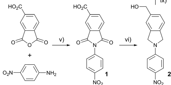
Scheme 2 (a) Reported synthetic route of TNQ-ZnP-TAPD using the protected TAPD precursor 3 . 7a,b (i) \text{BF}_3 \cdot \text{OEt}_2 , \text{DCM} then \text{DDQ} ; (ii) \text{SnCl}_2 , \text{HCl} ; (iii) \text{NaBH}_3\text{CN} , \text{CH}_2\text{O} ; (iv) \text{Zn}(\text{OAc})_2 , \text{CHCl}_3/\text{MeOH} ; (b) new synthesis of 3 . (v) \text{AcOH} , 12 h, 118 °C, 95%; (vi) \text{BH}_3 \cdot \text{THF} , \text{THF} , 12 h, 66 °C, 75%; (vii) activated \text{MnO}_2 , \text{CHCl}_3 , 15 min, 25 °C, 70%.
