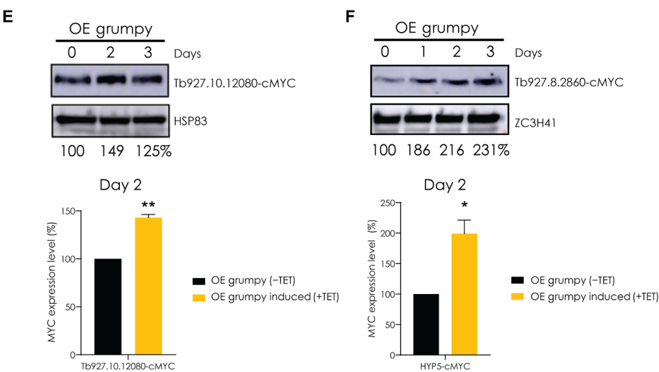
Fig. 8. snoGRUMPY interacts with stumpy-related transcripts and regulates their expression. (A) Top 10 mRNA targets of snoGRUMPY identified using in vivo psoralen ultraviolet (UV) cross-linking. Results are shown as the total number of reads sequenced that match the specific target gene. (B to F) Tb927.10.12080 is an mRNA target of snoGRUMPY . (B) Growth curve of parasite overexpressing Tb927.10.12080 gene alone (light blue) or together with grumpy (dark blue). Results are shown as means (SEM, n = 3 ), statistical test: two-way ANOVA (Dunnett's multiple comparisons test), adjusted P values: *P < 0.05 ; ****P < 0.0001 . WT, wild-type. (C) Percentage of GFP::PAD1-positive parasites (stumpy forms) measured by FACS in parasite overexpressing Tb927.10.12080 gene alone (dark green) or together with grumpy (light green). Statistical test: two-way ANOVA (Tukey's multiple comparisons test), adjusted P value: ****P < 0.0001 . (D) RNA-FISH showing the localization of Tb927.10.12080 mRNA (green) and grumpy lncRNA (red), in parasite overexpressing Tb927.10.12080 together with grumpy . The white arrow shows the colocalization of signal between Tb927.10.12080 mRNA and grumpy lncRNA. (E) Change in Tb927.10.12080 protein expression in grumpy -overexpressing cell line is analyzed by Western blot and normalized by the expression of housekeeping protein HSP83 (in procyclic forms). (F) Change in HYP5 (Tb927.8.2860) protein expression in grumpy -overexpressing cell line is analyzed by Western blot and normalized by the expression of housekeeping protein HSP83 (in procyclic forms). Statistical test for (E) and (F): two-tailed paired t test ( *P < 0.05 ; **P < 0.01 ).
