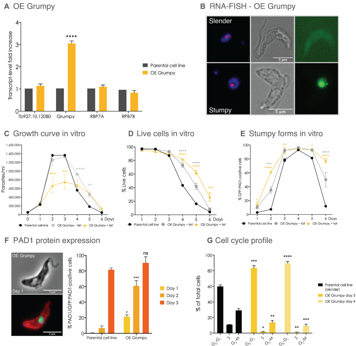
Fig. 5. grumpy overexpression promotes premature parasite differentiation. (A) Transcript levels measured by RT-qPCR of grumpy and its neighboring genes in parental cell line (black bars) and in grumpy -overexpressing (OE) cell line, 24 hours after tetracycline induction (yellow bars). Changes in transcript levels were measured by normalizing transcript level to a control gene (Tb927.10.12970) and to the parental cell line. (B) Subcellular localization of grumpy after overexpression using RNA-FISH. Left to right: GRUMPY , grumpy signal using RNA-FISH; phase-contrast signal of T. brucei parasite; GFP, GFP::PAD1 signal expressed in the nucleus of stumpy forms. (C to F) After inducing grumpy overexpression, we measured (C) parasite growth for 6 days (without passage), (D) percentage of live cells measured by fluorescence-activated cell sorting (FACS) of propidium iodide-stained cells, (E) percentage of GFP::PAD1-positive parasites (stumpy forms) measured by FACS, (F) percentage of parasites expressing both GFP::PAD1 and endogenous PAD1 protein that are measured by microscopy and image quantification. Microscopy picture (on the left) shows an example of a parasite expressing both GFP::PAD1 in the nucleus (in green) and the endogenous PAD1 protein at the cell surface (in red). Parasite DNA stained with 4',6-diamidino-2-phenylindole (DAPI) (in blue). (G) Cell cycle profile of parental cell line (slender forms) and grumpy -overexpressing parasites at days 3 and 4 of in vitro culture without passage. All results are shown as means (SEM, n = 3 ). Multiple t tests (A) and Sidak's multiple comparisons test (C to G) are used for statistical analysis using the parental cell line as the control for comparison (adjusted P values: * P < 0.05 ; ** P < 0.01 ; *** P < 0.001 ; **** P < 0.0001 ).
