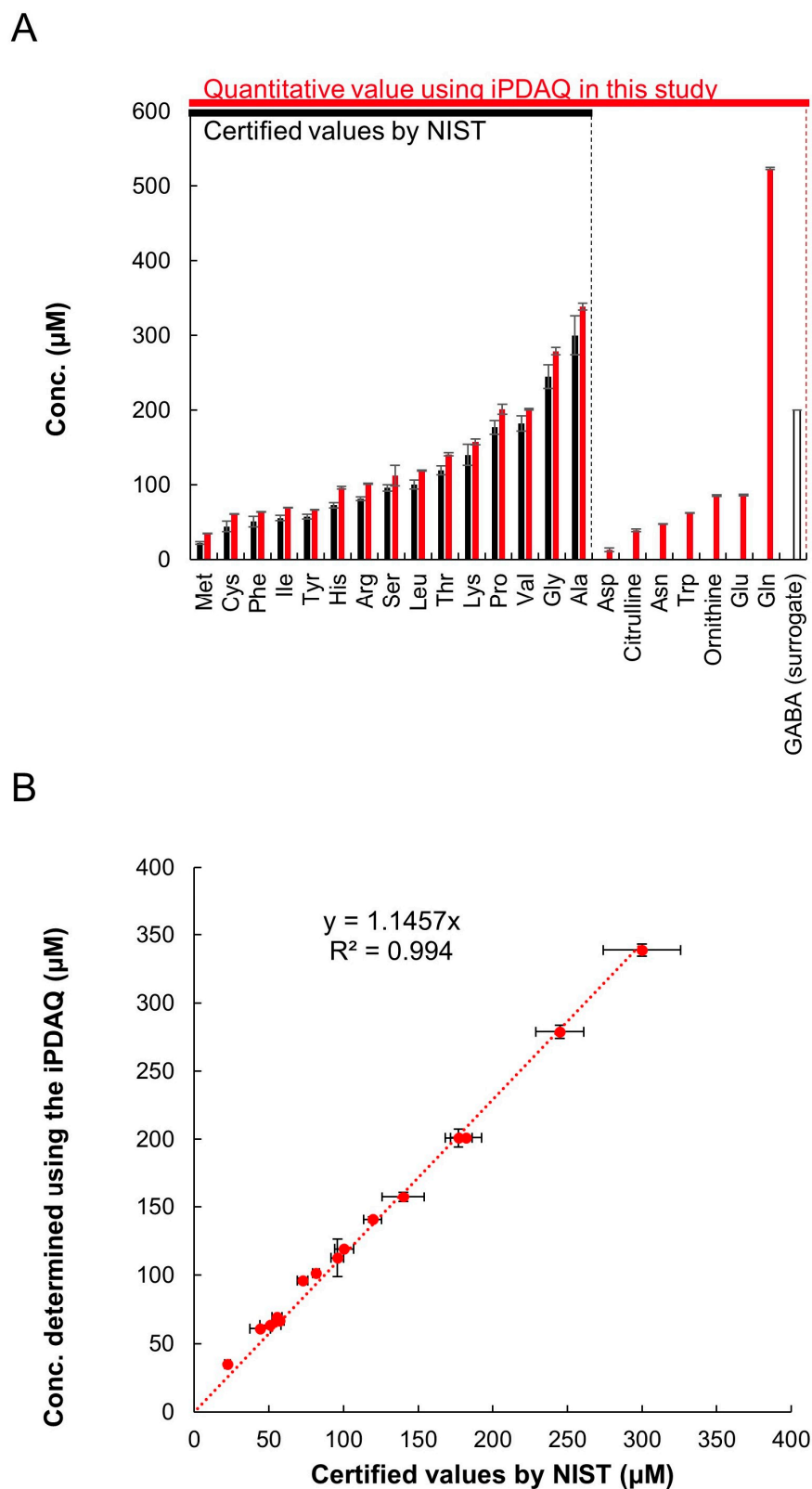
Figure 4. iPDAQ method validation using reference human plasma sample SRM1950. (A) Amino acid concentration in SRM1950. Black bars, certified amino acid concentrations provided by NIST. Red bars, amino acid concentration quantified using the iPDAQ method. Open bar, GABA used as a surrogate. (B) Comparison of the amino acid concentrations determined using the iPDAQ with the certified values provided by NIST. Error bars indicate the standard deviation ( n = 3 ).
