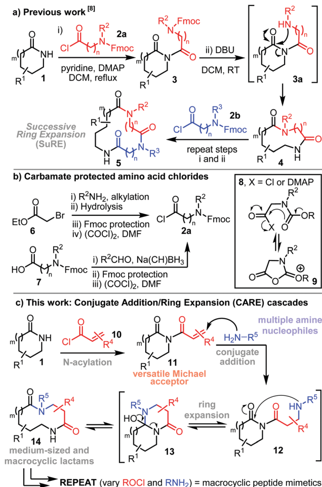
Scheme 1 Lactam ring expansion reactions.
