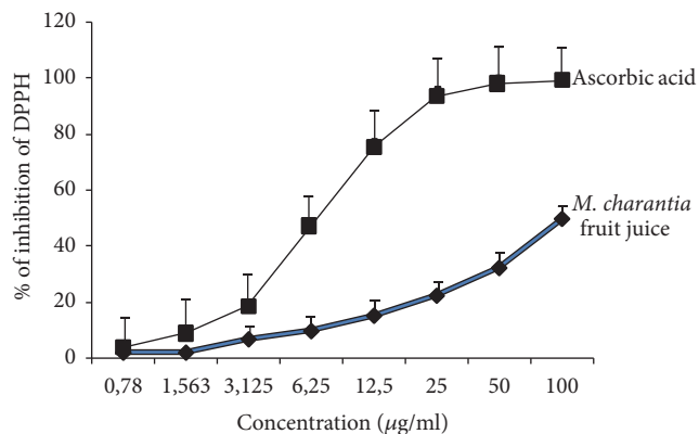
FIGURE 3: Antioxidant activities of Momordica charantia fruit juice. Values are means \pm SEM. Antioxidant capacity of plant fruit juice was determined in a solution of fruit juice (0.78–100 \mu\text{g/ml} ) as described in the Materials and Methods . Each value represents the mean of three determinations.
