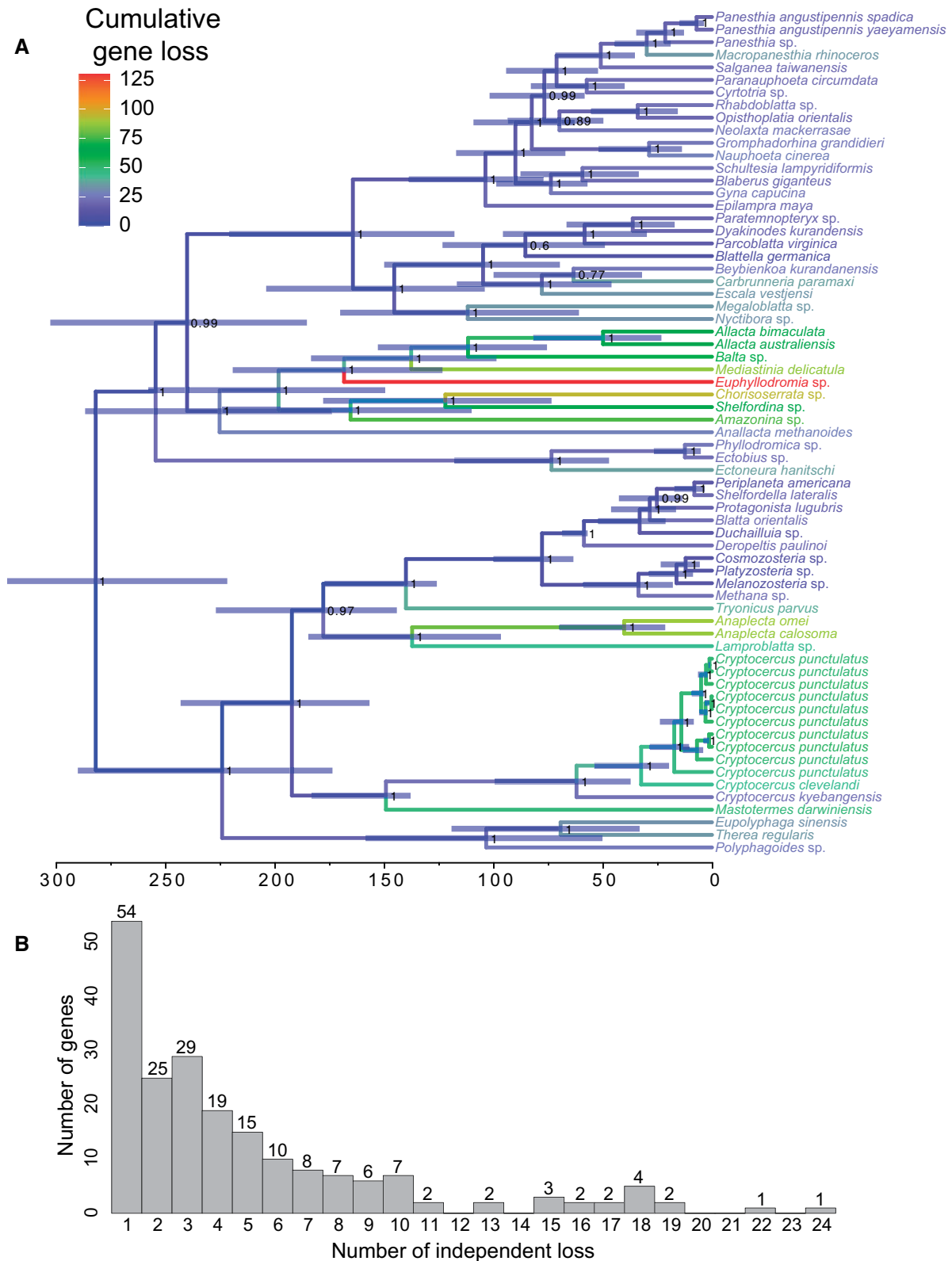
FIG. 1. Evolution of genome reduction by gene loss in Blattabacterium . (A) Time-calibrated phylogenetic tree showing the evolution of genome reduction by gene loss in Blattabacterium . The tree was reconstructed with BEAST, using a set of 31 marker protein-coding genes, with third codon position excluded (see Bourguignon et al. 2020). Branch color represents cumulative gene loss. Node labels represent posterior distribution. Node bars indicate 95% highest posterior density. (B) Histogram representing the frequency of independent gene loss estimated from the 200 protein-coding genes lost in at least one lineage. The numbers above each bar indicate the frequency of independent gene loss. Values were derived from the reconstruction of gene loss on the maximum likelihood phylogenetic tree with branch length and were rounded to the nearest integer.
