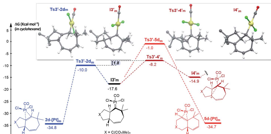
Fig. 7 Gibbs energy profile for the reaction of 1d catalyzed by \text{PtCl}_2(\text{CO}) in cyclohexane; energy of 1m (Fig. S15 † ) is considered as the reference. The gem-diesters [ X = \text{C}(\text{CO}_2\text{Me})_2 ] are omitted for clarity. See Fig. S15 and S16 † for the entire energy profile. 22
