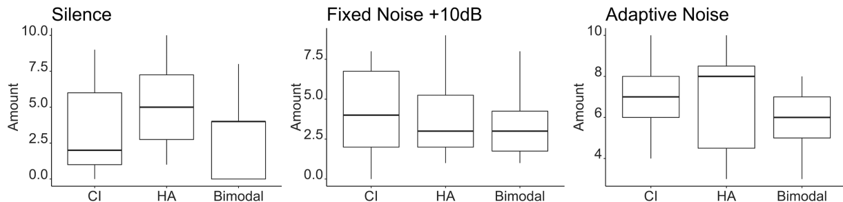
Fig. 1 Medians and first and third quartiles of the difficulty level using the Visual Analog Scale after performing the Hearing In Noise Test in the conditions of silence, fixed noise, and adaptive noise of each device and with bimodal stimulation. Abbreviation: CI: cochlear implant; HA: hearing aids
