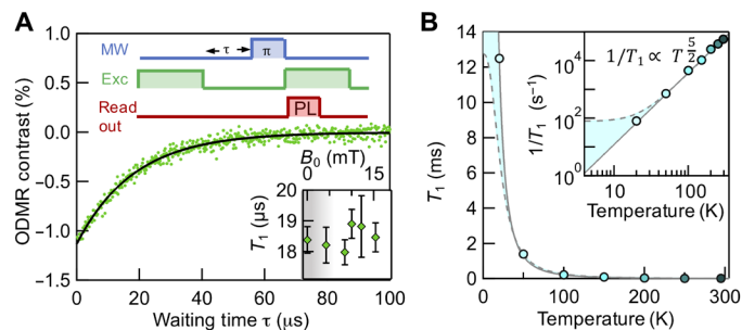
Fig. 2. Spin-lattice relaxation dynamics of V_B spin centers in hBN. (A) ODMR signal decay with waiting time \tau at T = 300 K. The pulse sequence is schematically shown, in which the duration of microwave \pi -pulse is known from Rabi experiments and the waiting time \tau is varied. Inset schematically shows T_1 versus external magnetic field (0 to 15 mT). The gray background indicates the magnetic field range where two ODMR transitions \nu_1 and \nu_2 overlap. (B) Temperature dependence of the spin-lattice relaxation time of V_B spin centers in hBN. The T_1 time increases by three orders of magnitude from 18 \mu s to 12.5 ms, when lowering the temperature to 20 K. Inset shows that a log-log plot for the spin-lattice relaxation rate ( 1/T_1 ) shows a T^{5/2} behavior over a broad temperature range. An upper boundary for the fastest spin-lattice relaxation rate can be estimated by assuming a saturation of the T_1 time at 20 K (highlighted in blue).
