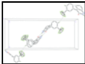
Fig. 2. Intermolecular hydrogen-bonding interactions (dashed lines) in the structure of (I). H atoms not involved in hydrogen bonding have been omitted.
