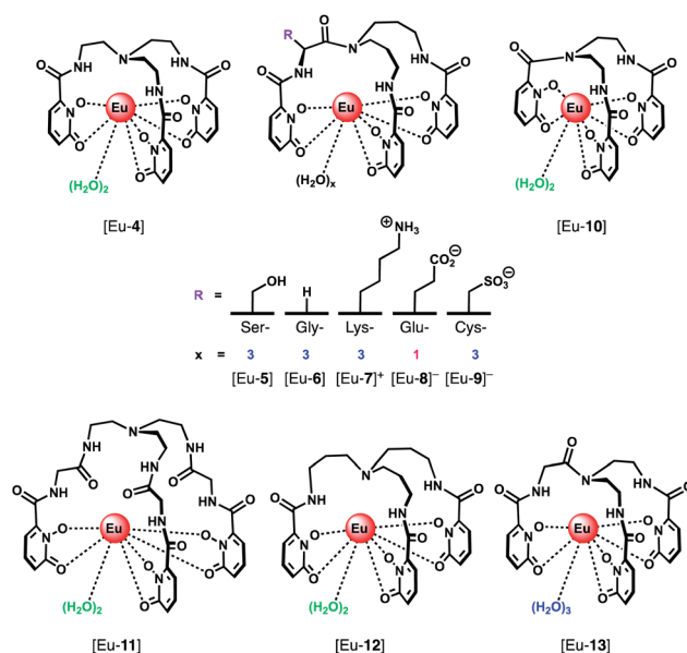
Fig. 5 Series of tripodal Eu(III) complexes evaluated for the selective detection of \text{HPO}_4^{2-} .
