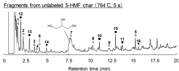
Fig. 5 Pyrogram obtained from the Py-GC/MS analysis (764 °C, 5 s hold time) of 5-HMF char generated by carbonization at 280 °C for 60 min.
