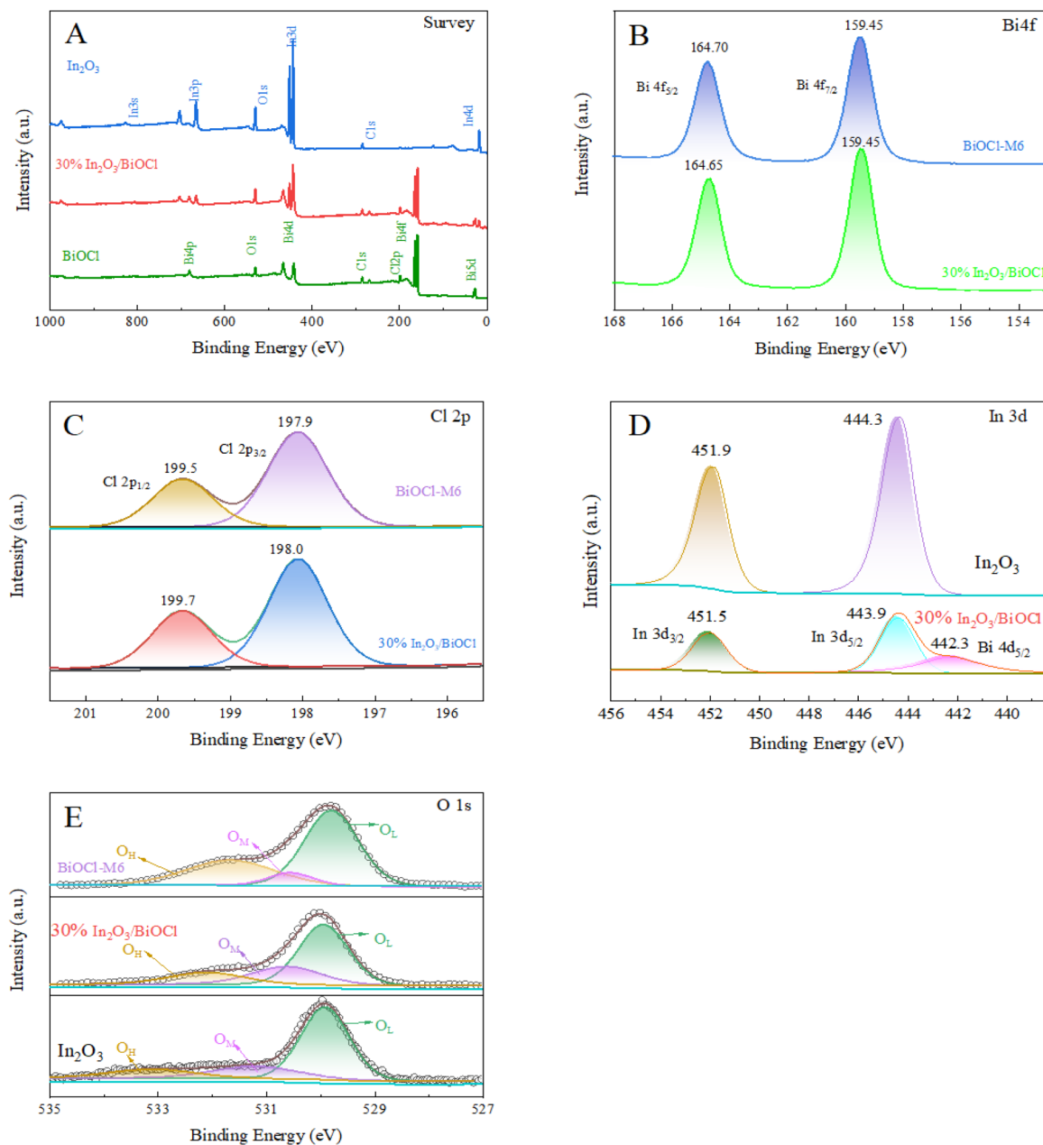
Fig. 5 XPS spectra of the photocatalysts. (A) XPS spectra of \text{BiOCl} , \text{In}_2\text{O}_3 , and 30% \text{In}_2\text{O}_3/\text{BiOCl} ; (B) Bi 4f spectra of \text{BiOCl} and 30% \text{In}_2\text{O}_3/\text{BiOCl} ; (C) Cl 2p spectra of \text{BiOCl} and 30% \text{In}_2\text{O}_3/\text{BiOCl} ; (D) In 3d spectra of \text{In}_2\text{O}_3 and 30% \text{In}_2\text{O}_3/\text{BiOCl} ; and (E) O 1s spectra of \text{BiOCl} , \text{In}_2\text{O}_3 , and 30% \text{In}_2\text{O}_3/\text{BiOCl} .
