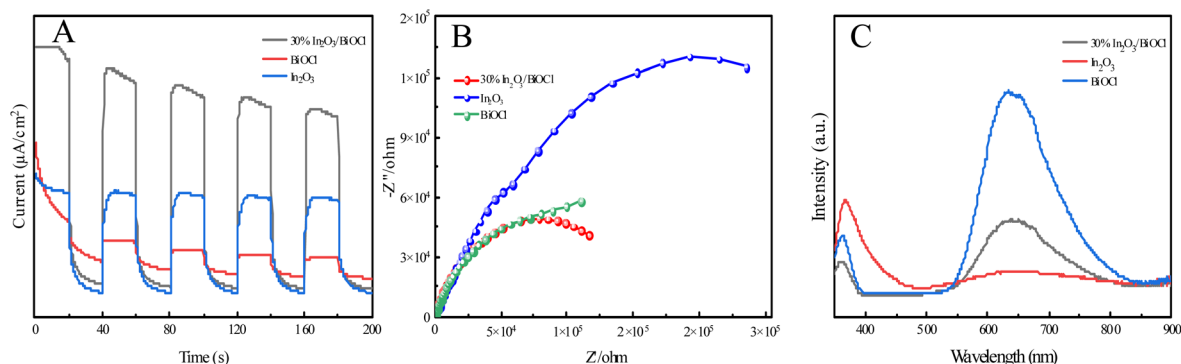
Fig. 14 (A) I-t spectra of (BiOCl, In 2 O 3 , and 30% In 2 O 3 /BiOCl); (B) EIS diagrams of (BiOCl, In 2 O 3 , 30% In 2 O 3 /BiOCl); (C) PL spectra of (BiOCl, In 2 O 3 , 30% In 2 O 3 /BiOCl).
