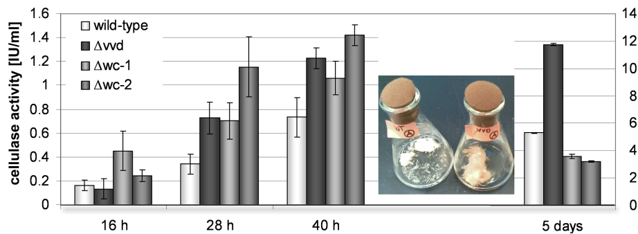
Figure 1 Secretion of cellulolytic enzymes by wild type, \Delta wc-1 , \Delta wc-2 and \Delta vvd mutants. Azo-CMC cellulase (endoglucanase) activity in culture filtrates of N. crassa wild type (WT) and mutant strains upon growth in Birds-medium with 2% (w/v) Avicel cellulose as sole carbon source at 16, 28 and 40 hrs versus 5 days. The flasks show examples for degradation of Avicel in wild type (left) and \Delta vvd mutant (right) strains after 40 hours of growth. At this timepoint the cellulosic substrate was almost or completely degraded by the strains used in this study. Error bars show standard deviation of at least three biological replicates.
