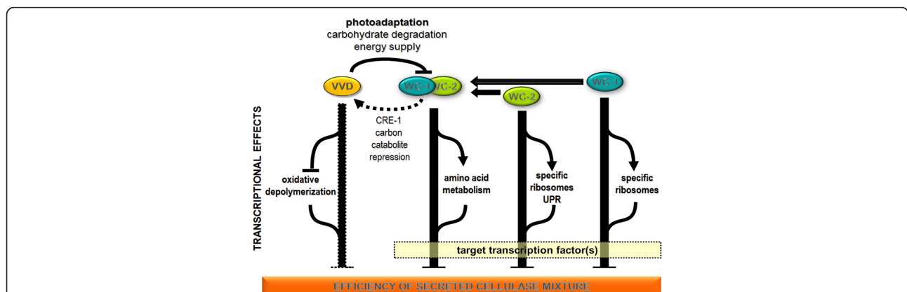
Figure 8 Model for regulation of plant cell wall degrading capacity in N. crassa by WC-1/WC-2/WCC and VVD. VVD, WC-1 and WC-2 negatively affect efficiency of cellulose degradation during early stages of growth. Regulation of cellulolytic enzymes and energy supply is subject to photoadaptation by WD, while carbon catabolite repression as mediated by CRE-1 is regulated by the WCC via VVD. Independent regulatory functions of VVD influencing cellulolytic efficiency include regulation of oxidative depolymerization, while for WC-1 and WC-2 these functions are most obvious in regulation of specific ribosomes. The WCC moreover specifically targets amino acid metabolism. Since the effect of the light response machinery is likely to be indirect, their output may involve additional target transcription factors.
