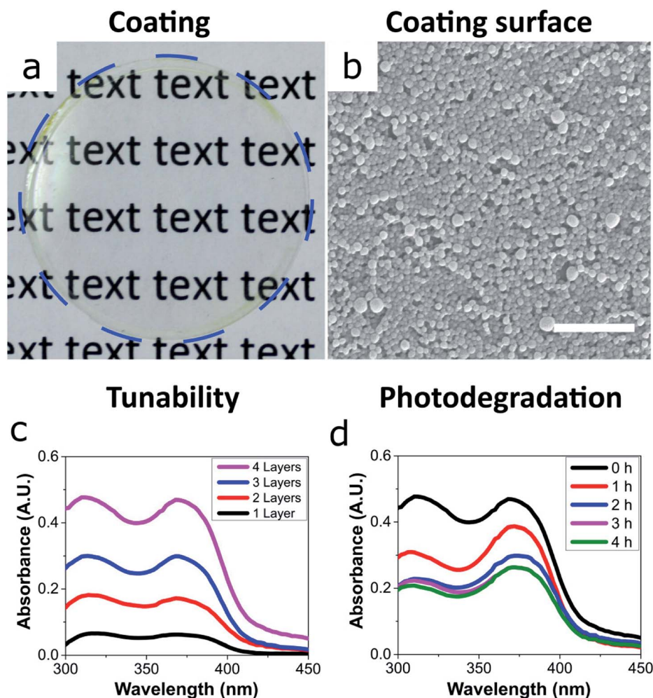
Fig. 2 (a) Photo of a transparent and uniform coating of the ECNPs on a glass cover slip. (b) SEM image of the coating surface, scale bar 1 \mu\text{m} . (c) Absorbance measurements of the ECNP coating showing the absorbance of each successive spin coated layer. Wavelengths lower than \lambda = 300 nm are not shown as they are absorbed by the glass coverslip. (d) Absorbance measurements showing the degradation of the absorbance of the 4-layer coating of ECNPs when irradiated by artificial sunlight for 4 h.
