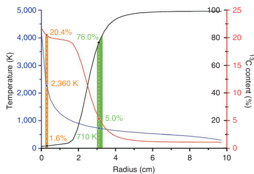
Figure 4 | Simulated curves of temperature and ^{13}C content. Simulated temperature (blue line) and ^{13}C content of carbon sources (black for Exp. B, red for Exp. C) versus distance from the arc centre (radius r ) for a reaction period of 600 s. Fullerenes with ^{13}C content of 1.6 \pm 0.1\% in Exp. B and 20.4 \pm 0.1\% in Exp. C are produced in an area of r \sim 2\text{--}3\text{ mm} at \sim 2,000\text{--}2,500\text{ K} (orange background) while a fraction of chloro-PAHs with ^{13}C content of 76.0 \pm 0.9\% in Exp. B and 5.0 \pm 0.4\% in Exp. C are produced in an area of r \sim 30\text{--}33\text{ mm} at \sim 700\text{--}730\text{ K} (green background).
