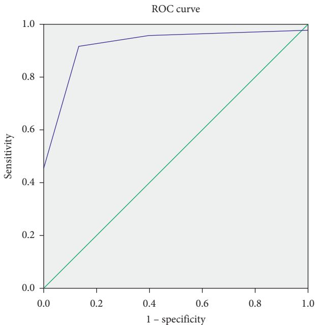
FIGURE 1: ROC curve. ROC curve in Section 3.3 showing a high value of sensitivity and specificity with larger area under the curve, and a steeper and sharper slope of the curve.
