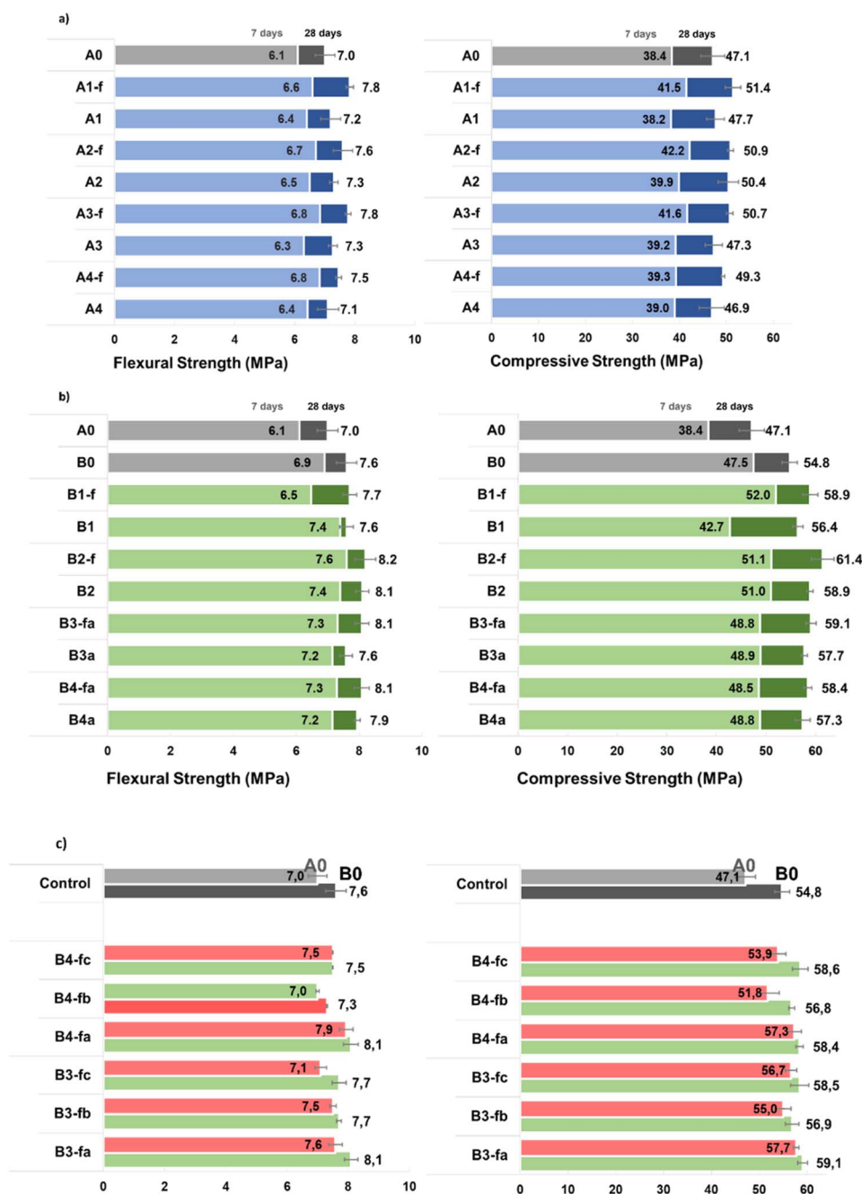
Fig. 5 Flexural and compressive strength values of mortar samples prepared with (a) 0.05% of GBM by weight of cement using Method A and measured after 7 and 28 days of curing; (b) 0.05% of GBM by weight of cement using Method B and measured after 7 and 28 days of curing; (c) 0.05–0.5% of GBM by weight of cement using Method B and measured after 28 curing days; the red bars refer to the mechanical performance of mortars containing pristine GBM 3 and 4, the green bars represent the performance of mortars containing functionalized GBM 3-f and 4-f. GBM content is highlighted in the final letter of the mortar code a = 0.05 w/w, b = 0.1\% w/w, c = 0.5\% w/w.
