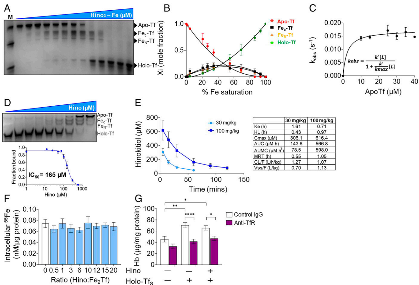
Fig. 4. Iron is transferred from hinokitiol to apotransferrin. (A and B) A total of 4 μM apo-Tf was incubated overnight with various concentrations of Fe(Hino) 3 to study the thermodynamics of iron transfer. [Apo-Tf]:[Fe-Hino] = 1: 0, 0.125, 0.25, 0.4, 0.5, 0.6, 0.8, 1, 1.25, 1.5, 2, 3, 4. (A) The first lane is a marker to denote various Tf species. Different Tf species were separated on a 10% tris-borate-ethylenediamine tetraacetic acid urea gel. (B) Mole fractions of the corresponding Tf-Fe complexes formed at each apo-Tf: Fe(Hino) 3 ratio were graphed according to SI Appendix, Appendix S1 . Results are means ± SEM ( n = 3 to 4 samples/group) from two independent experiments. (C) Pseudo first kinetic rate constants ( k obs ) at various apo-Tf concentrations were graphed according to SI Appendix, Appendix S2 . Results are means ± SEM from 5 to 6 independent experiments. (D) Titration of 12.5 μM holo-Tf with various concentrations of hinokitiol was measured using urea gel. Results are means ± SEM ( n = 3 samples/group). Two independent experiments were performed yielding similar results. (E) Pharmacokinetics of hinokitiol in mice following IP injection of 30 mg/kg or 100 mg/kg hinokitiol and its pharmacokinetic parameters. Abbreviations: k e , elimination rate constant; HL, half-life; C max , maximum concentrations; AUC, area under the plasma concentration-time curve; AUMC, area under the first moment curve; MRT, mean residence time; CL/F, apparent clearance after extravascular administration; V ss /F, volume of distribution after extravascular administration. Results are means ± SEM ( n = 3 samples/group). At least two independent experiments were performed yielding similar results. (F) Intracellular 55 Fe levels in MEL cells pulsed with 0.165 μM 55 Fe 2 Tf and treated with various biologically-relevant ratios of [hinokitiol]:[Fe 2 Tf]. Results are means ± SEM ( n = 8 samples/group). Three independent experiments were performed yielding similar results. (G) Hemoglobin level measured in MEL cells differentiated with 5 μM holo-Tf 5 in the presence of 1 μM hinokitiol (+) behaved similarly to no-hinokitiol-treated (-) group. Results are means ± SEM ( n = 3 samples/group) from at least three independent experiments performed in triplicate. * P < 0.05, ** P < 0.01, and **** P < 0.0001 by two-way ANOVA with Tukey's multiple comparison test.
