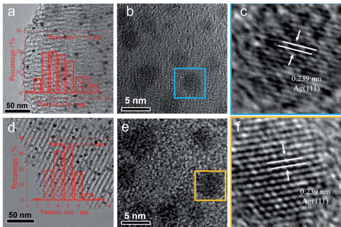
Fig. 2 TEM images and HRTEM images of typical regions determined from 5\text{Ag}_1\text{-Li}_{0.05}/\text{SBA-15} catalysts (a–c) compared to 5\text{Ag}/\text{SBA} (d–f), accompanied by the corresponding average particle size (inset image) and lattice fringes of Li-free and -doped silver nanoparticles.
